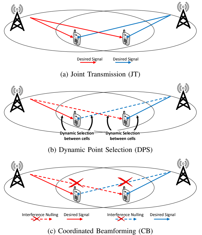
Figure 2: Main Downlink CoMP Types for LTE-A [7]
