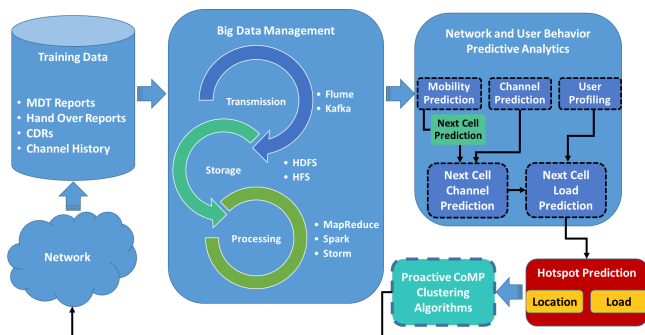
Figure 7: Big Data Empowered Proactive CoMP Clustering Framework
