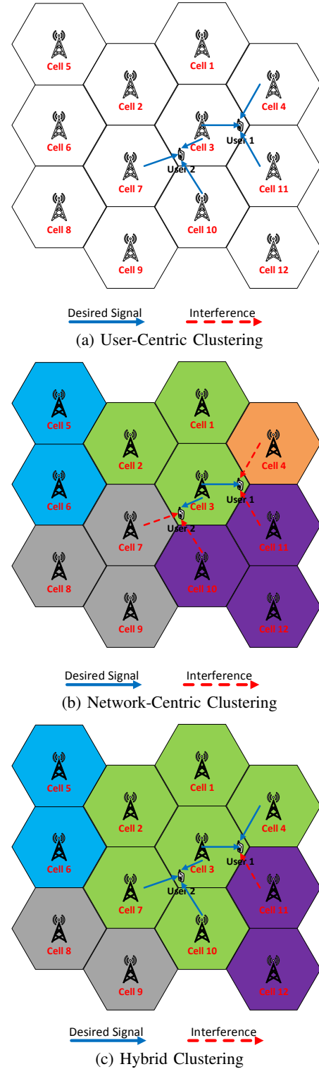
Figure 5: Dynamic CoMP Clustering Taxonomy
