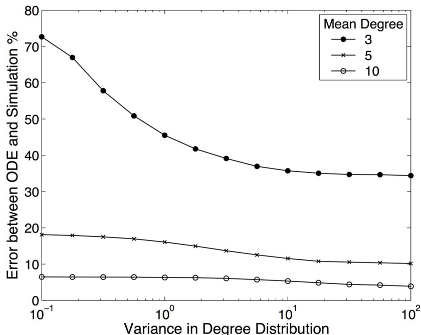
Fig 1. Comparison between risk-structured mean-field results and stochastic network simulations for SIS infection dynamics. The error is the relative percentage error between the risk-structured mean-field model (Supporting Information) and network simulation results for the mean prevalence of infection: Error = 100 \times \|I_{ODE} - I_{network}\| / I_{network} . The degree distribution obeys P(k) = \rho \exp(-\alpha(k - K)^2) for all k \geq 2 , where \alpha and K are determined to give a desired mean and variance, and \rho is a normalising constant. Other methods of generating degree distributions give similar results. We insist on k \geq 2 (for all nodes) as this generally ensures that the majority of network form a single giant component. The network is formulated using the Molly-Reed algorithm [47] with 100,000 nodes, but ensuring that there were no self-contacts and no multiple connections between individuals. We assume the recovery rate of individuals \gamma is scaled to be one, while the transmission rate across a contact scales with the mean number of contacts, \tau = 2/\bar{k} . As such, the mean prevalence in both simulation and ODE models lies between 30 and 50%.
