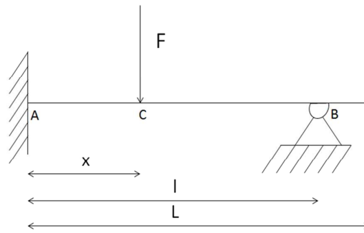
Figure 1. Mechanical model of the switch blade lateral behaviour.
