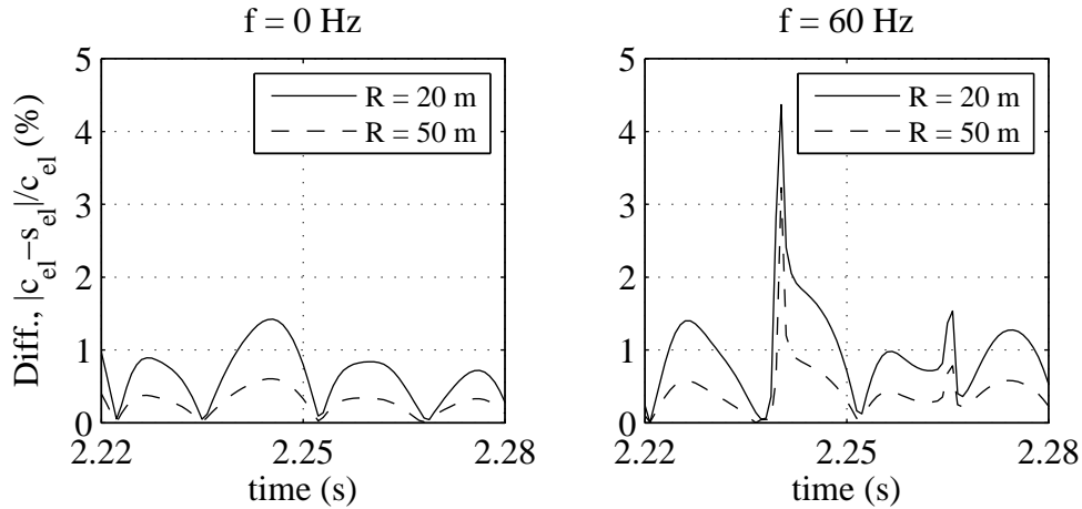
Figure 7: Percentage difference for the vertical displacement between using curved and straight elements for a track of length L_t = 90\text{ m} subjected to a load with speed V = 20\text{ m/s} .
