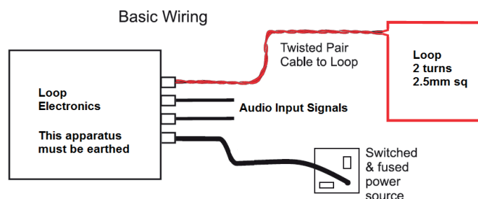
Figure 4 Basic Wiring
