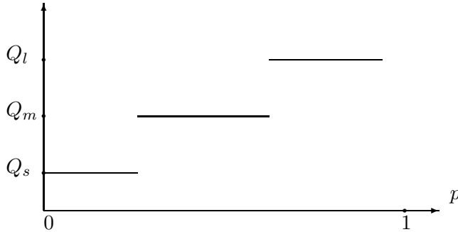
Figure 3. The figure depicts a provision rule with three bunching regions.
