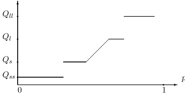
Figure 2. The figure depicts a provision rule with four bunching regions. Over an intermediate range the provision rule is strictly increasing and coincides with the modified Samuelson Rule, Q^* . The graph assumes a quadratic cost function so that Q^* is linear in p .
