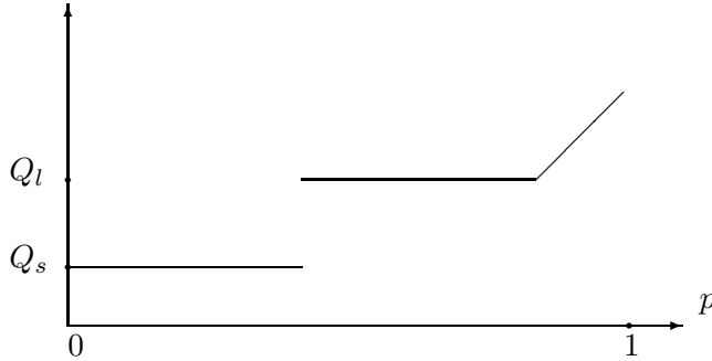
Figure 5. The figure depicts a provision rule with two bunching regions. For large p the provision rule is strictly increasing and coincides with the modified Samuelson Rule, Q^* .
