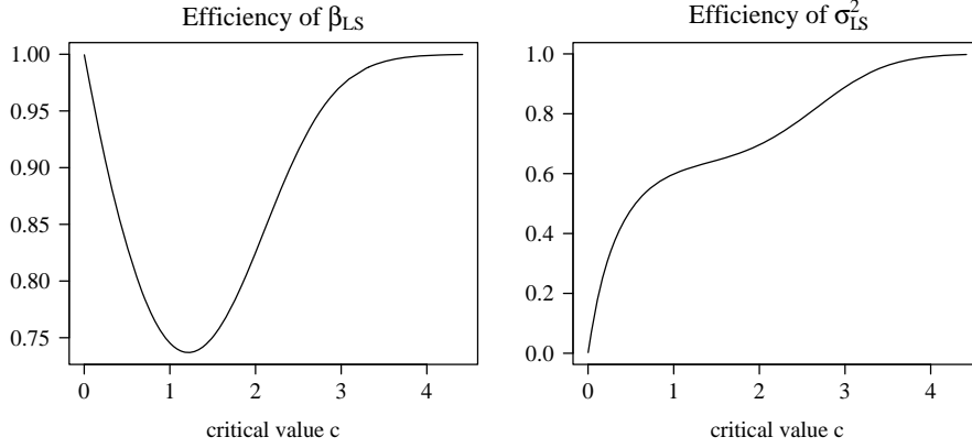
Figure 1: The efficiency of the estimators \check{\beta}_{LS} and \check{\sigma}_{LS}^2 with respect to the least squares estimators \hat{\beta} and \hat{\sigma}^2 , respectively, for f equal to the Gaussian density.
