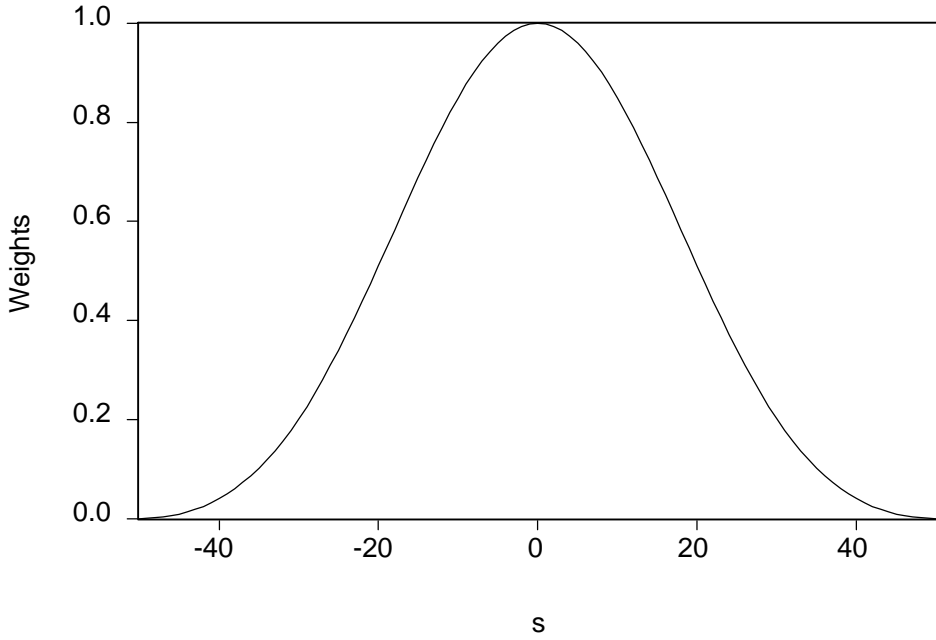
Figure A1 - Weight Function for Blackman-Tukey Window with M=50
