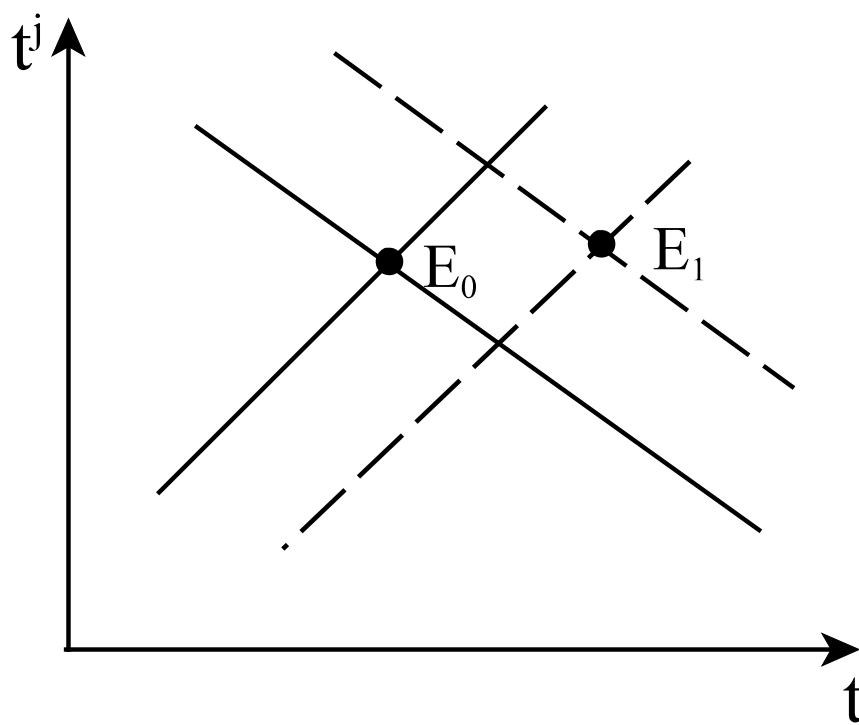
Figure 5: NE, \theta > 1 , \theta^j < 1
