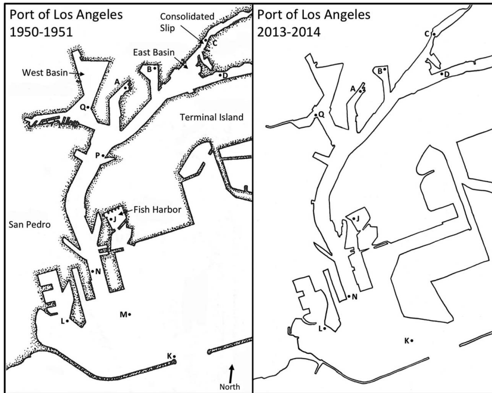
Fig. 1a. Map of Los Angeles—Long Beach Harbors showing the station locations in the Los Angeles Harbor survey conducted in 1950-1951. 1b. Map of Los Angeles Harbor showing the station locations in the 2013-2014 survey.
