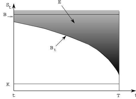
FIGURE 1.4.2. Exercise Region for a Standard American Option
