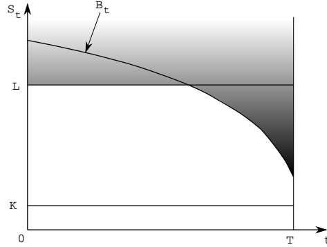
FIGURE 1.5.2. Exercise Region for an American Capped Call Option
