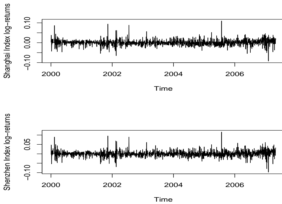
Fig. 1. Log-returns for Shanghai Stock Composite Index and Shenzhen Stock Composite Index from 4 January 2000 to 29 May 2007
