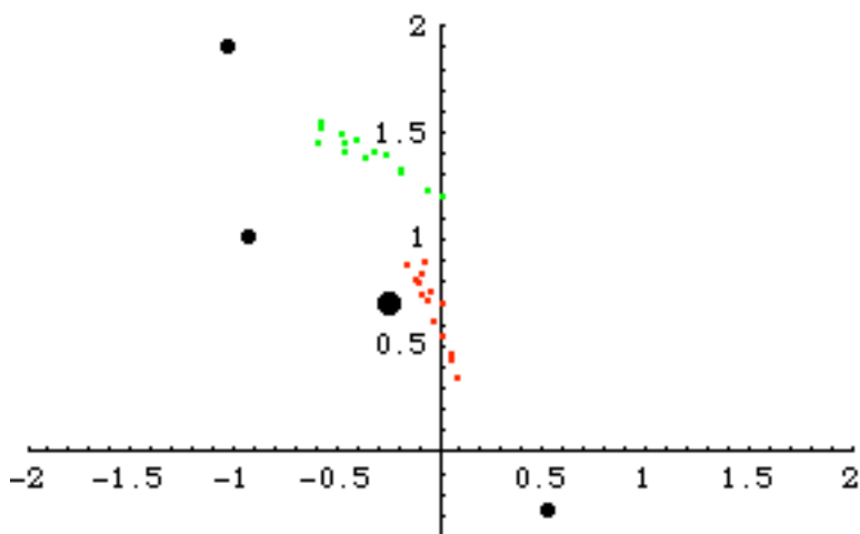
Figure 3b PUNEs, 2001, \beta=0.65 . See legend for figure 3a.
