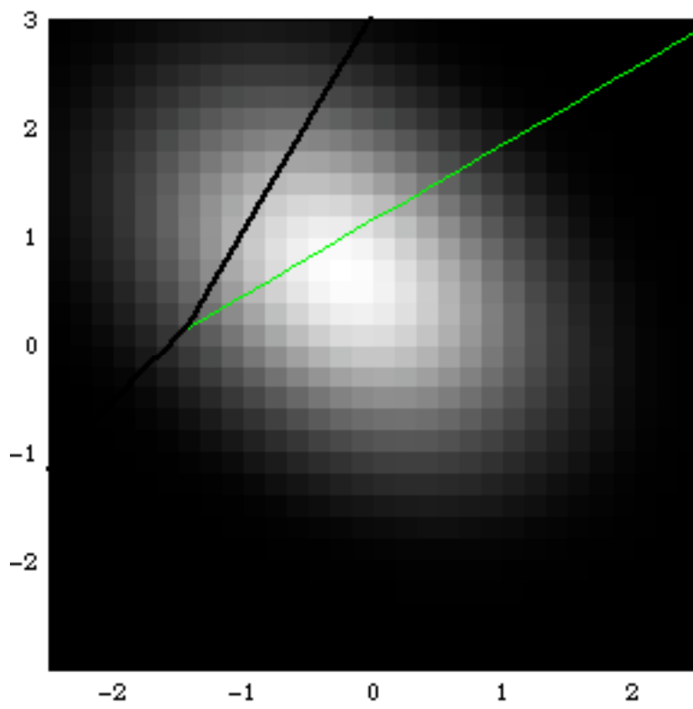
Figure 4b Partition of type space into three party constituencies, 2001, \rho=0.65
