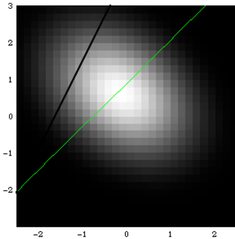
Figure 4a Partition of type space into three party constituencies, 1998, \rho=0.6
