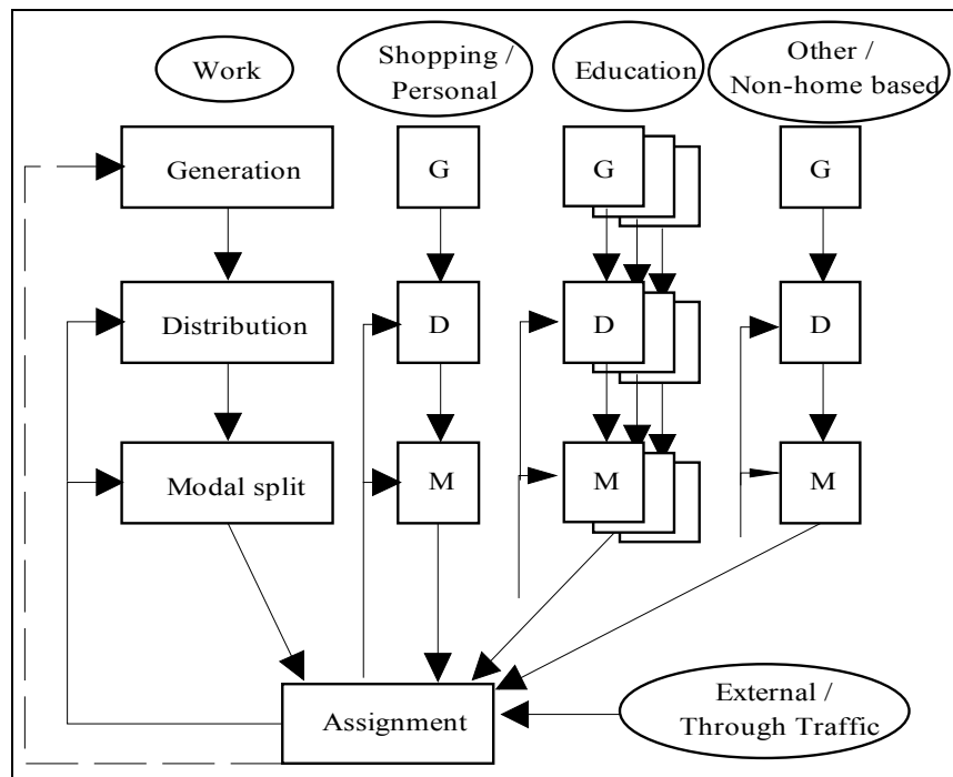
Figure 1. The model architecture
