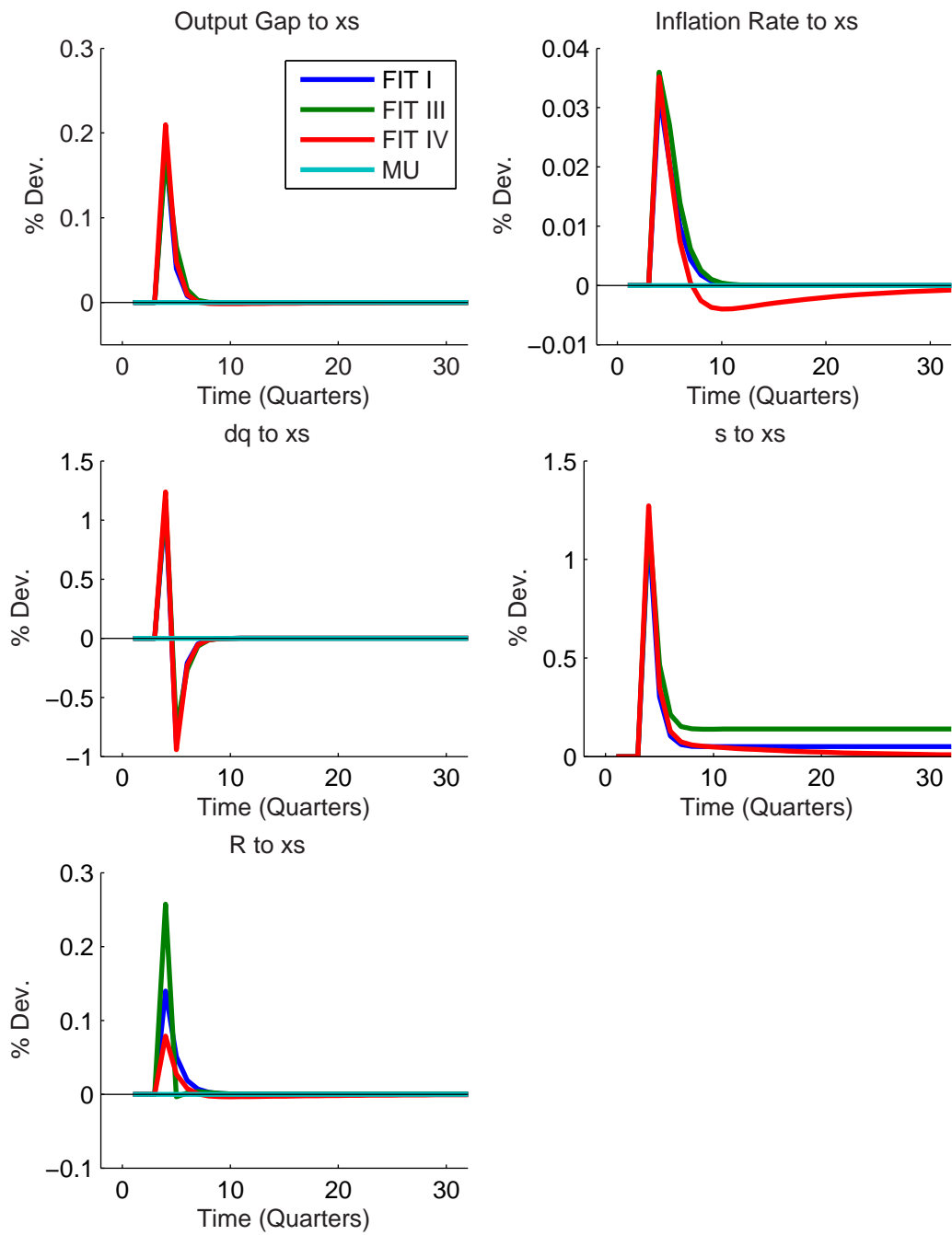
Figure 3: Impulse Responses of Domestic Variables to UIP Shock (MN)
