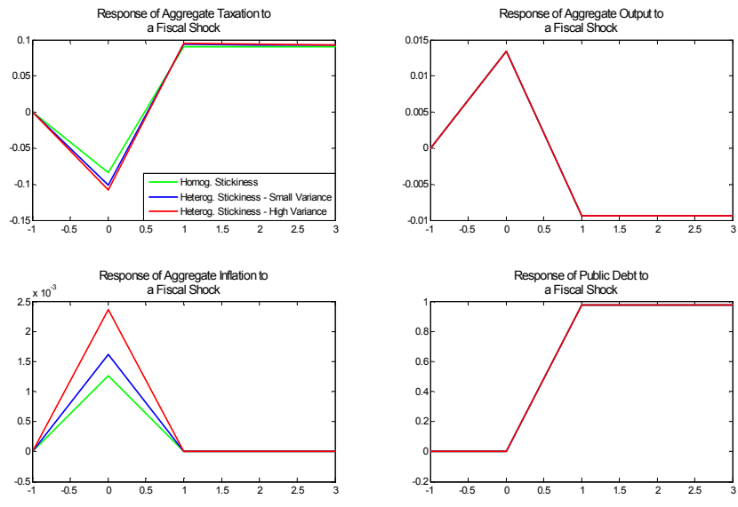
Figure 5: Effects of a Fiscal Shock on Aggregate Variables: Homogeneous Taxation Case.
