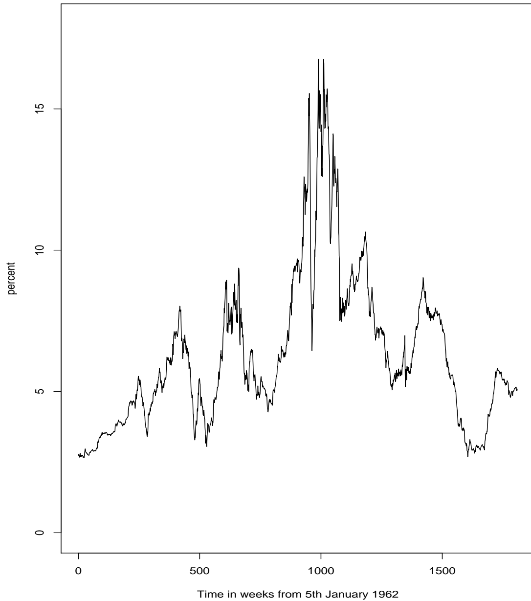
Figure 5: Weekly 3-month US Treasury bill rate from the 5th of January 1962 up to the 30th of August 1996.
