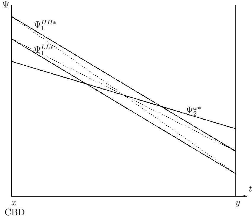
Figure 1: The bid rent functions in Example 1, where the dotted lines represent \Psi_1^{HL*} and \Psi_1^{LH*} , respectively.
