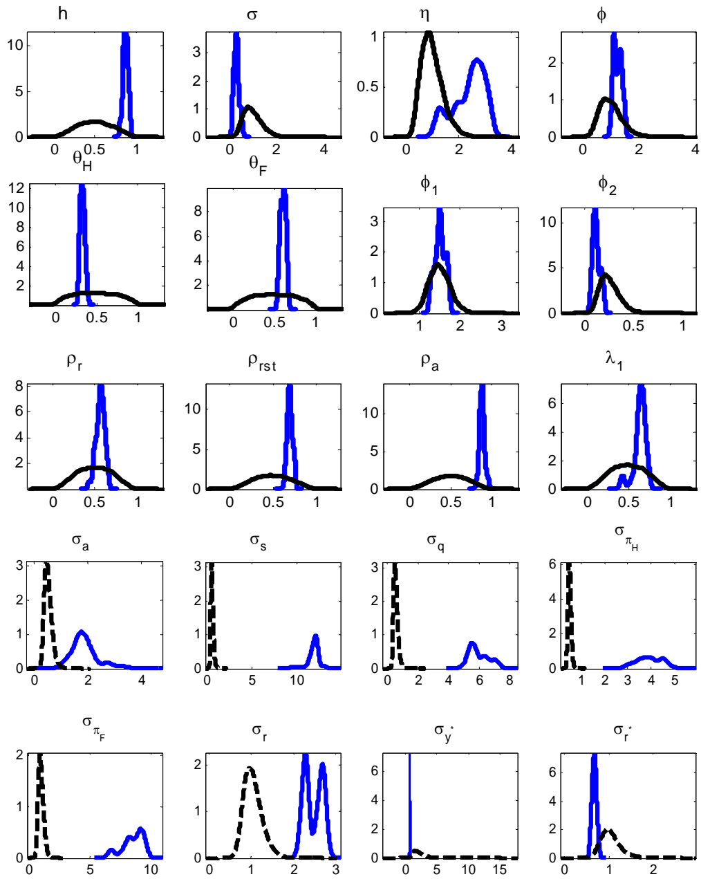
Figure B1: Model Prior and Posterior Distribution Plots
