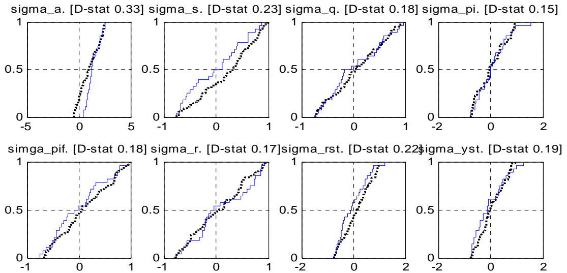
(b) Stability plots for Model Structural Shocks
