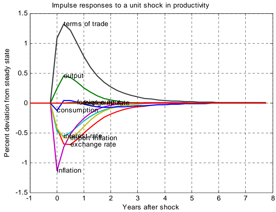
Figures B3: DSGE Model Impulse-responses Functions
