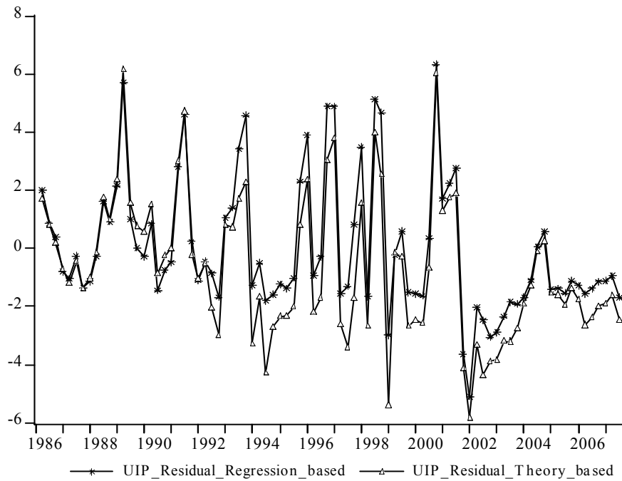
Figure A4: Uncovered Interest Parity Condition Residuals
