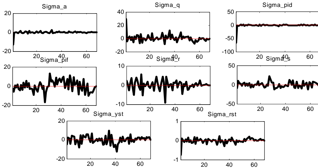
Figure B5: Smoothed Shocks
