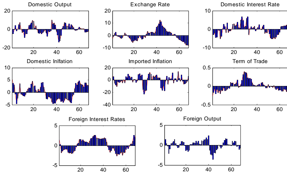
Figure B4: Historical Smoothed Variables 30
