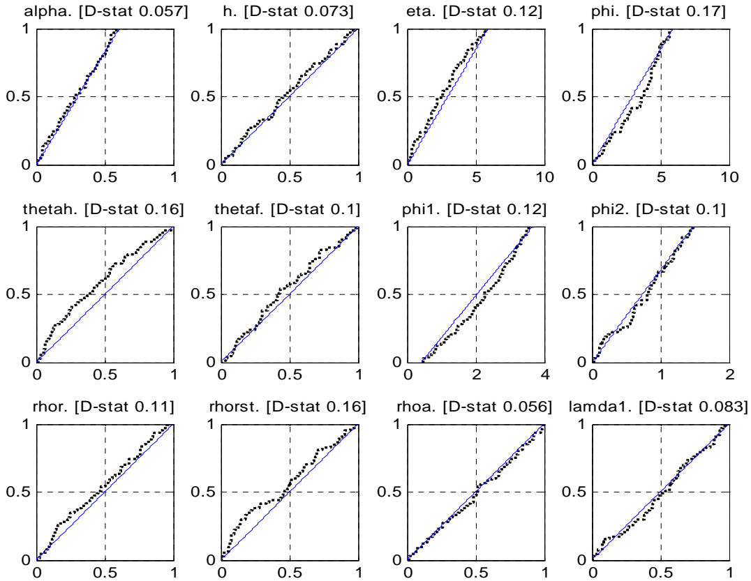
(a) Stability Plots for Model Structural Parameter
