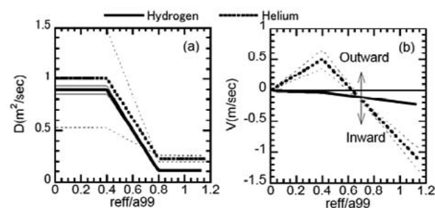
Fig.3 Comparison of (a) diffusion coefficients and (b) convection velocities. Thin lines are upper and lower bounds of fitting error
