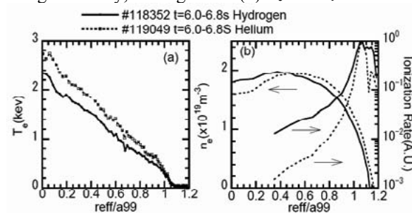
Fig2 Comparison of profiles (a) T_e (b) n_e and ionization rate. T_e profiles are from Thomson scattering and n_e profiles are from FIR interferometer
