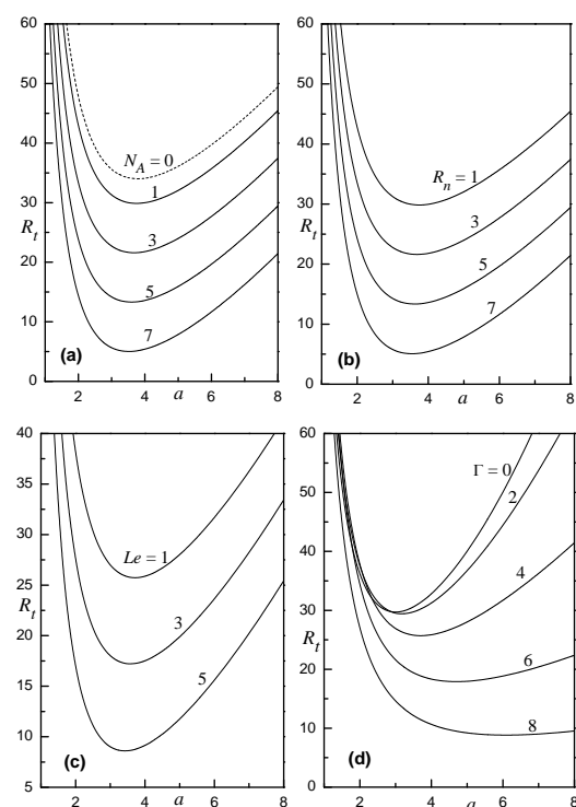
Fig. 2: Neutral curves for different values of (a) N_A with R_n = 2 , N_B = 0.059 , Le = 1 and \Gamma = 4 (b) R_n with N_A = 2 , N_B = 0.059 , Le = 1 , \Gamma = 4 (c) Le with R_n = 2 , N_A = 2 , N_B = 0.059 , \Gamma = 4 (d) \Gamma with Le = 1 , R_n = 1 , N_A = 4 , N_B = 0.059
