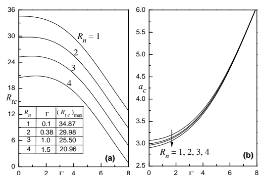
Fig. 4: Variation of (a) R_{tc} , (b) a_c with \Gamma for different values of R_n when Le=1 , N_A=2 and N_B=0.059 .
