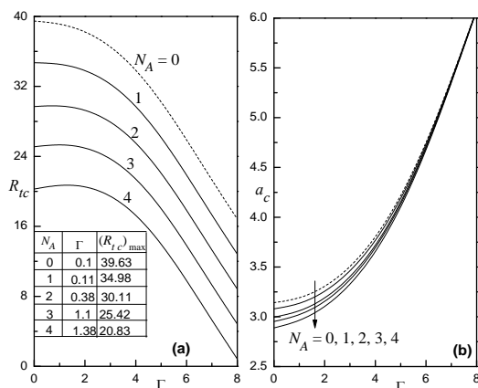
Fig. 3: Variation of (a) R_{tc} , (b) a_c with \Gamma for different values of N_A when Le=1 , N_B=0.059 and R_n=2
