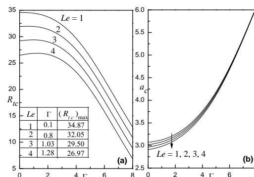
Fig. 6: Variation of (a) R_{tc} , (b) a_c with \Gamma for different values of Le when N_B=0.059 , N_A=2 and R_n=1
