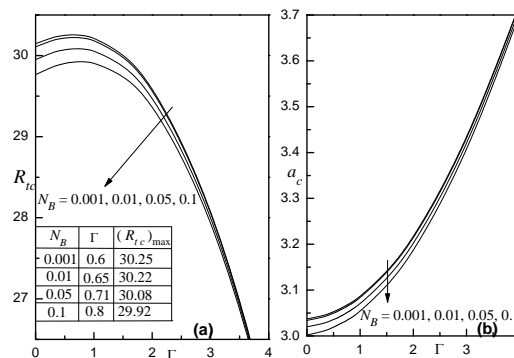
Fig. 5: Variation of (a) R_{tc} , (b) a_c with \Gamma for different values of N_B when N_A=2 , R_n=2 and Le=1
