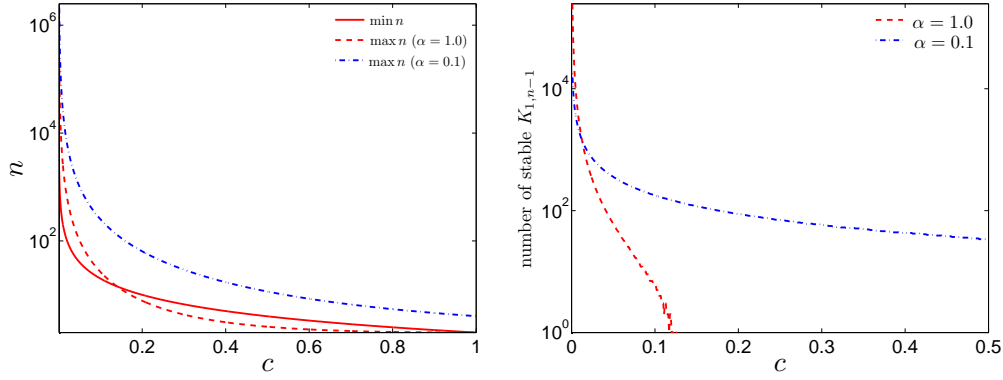
Fig. 16. Upper and lower bounds for the sizes of the stars (left) and the number of stars of different sizes (right) for \alpha = 1 and \alpha = 0.1 . One can see that for \alpha = 1 and cost larger than 0.4 a stable spanning star does not exist.
