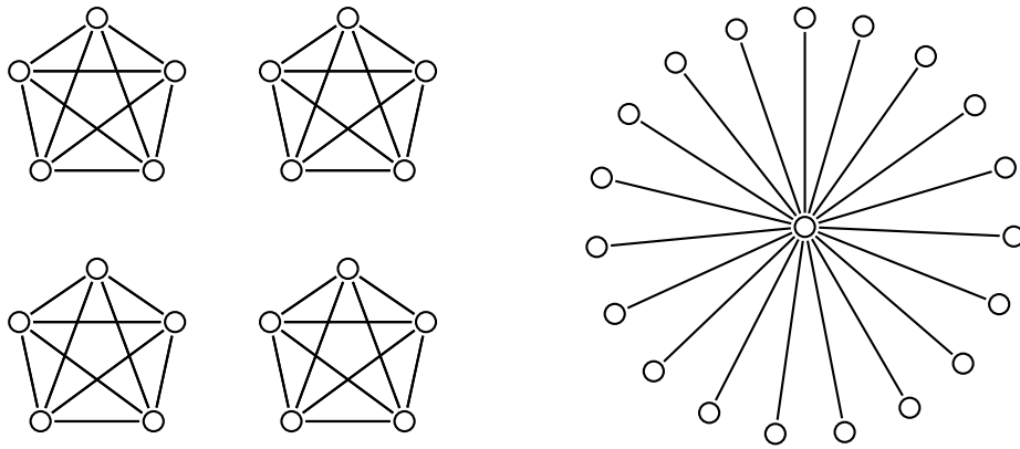
Fig. 7. An example of two possible (different) equilibrium networks for cost c = 0.3 and \alpha = 0.1 with n = 20 firms. A set of disconnected cliques of the same size (left) and a spanning star (right)
