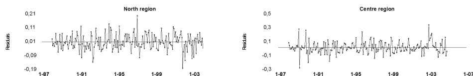
Graph of the residuals for model M1, for the two regions
