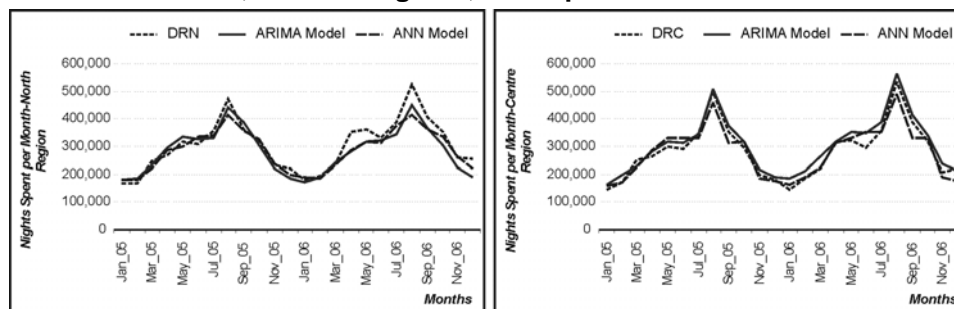
Original Nights Spent and Prediction Tourism Demand with ARIMA and ANN models, for both regions, in the period 2005:01 to 2006:12
