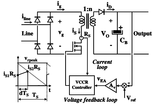
Fig.8: Flyback PFC with VCCR Control.
