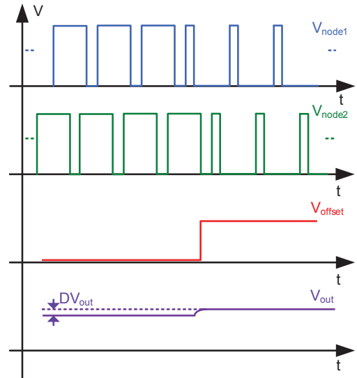
Fig. 8: Ideal transition between levels in the Floating Two-phase Buck
