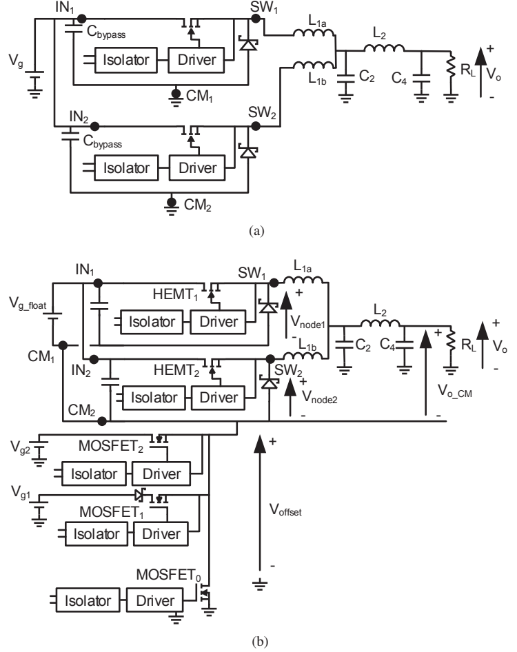
Fig. 4: Combinations with the switch cell: (a) Two-phase Buck with 4 th order filter, (b) Floating Two-phase Buck with 4 th order filter
