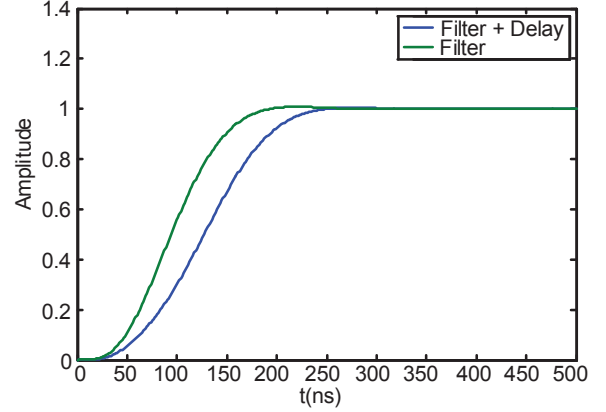
Fig. 10: Step responses of the combination of the delay and G_{filter} ( G_{two-phases} ) and only G_{filter}
