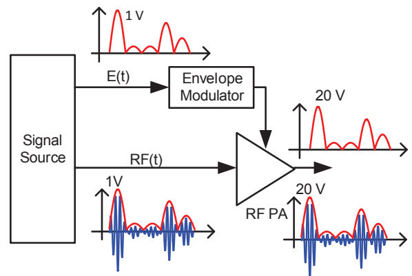
Fig. 1: Envelope Tracking Architecture
