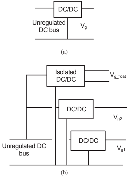
Fig. 6: (a) Power supply architecture for the Two-phase Buck (b) Power supply architecture for the Floating Two-phase Buck
