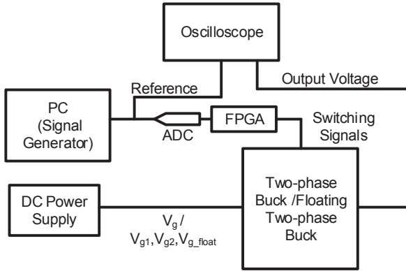
Fig. 14: Scheme of the experimental set up
