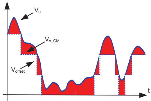
Fig. 5: Explanation of voltages in the Floating Two-phase Buck converter
