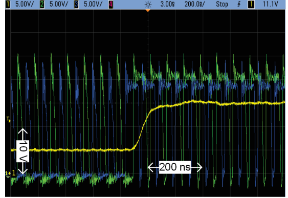
Fig. 15: Step response of the Two-phase Buck converter
