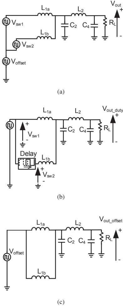
Fig. 9: Equivalent circuits to study the transitions: (a) Equivalent circuit, (b) Equivalent circuit for transients only in the duty cycle, (c) Equivalent circuit for transients only in the offset voltage
