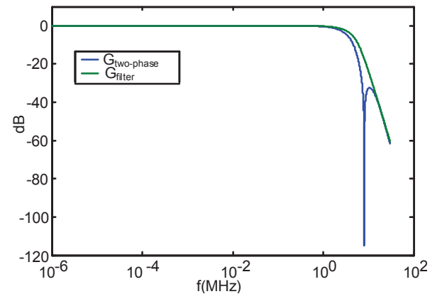
Fig. 7: Bode plot of a 4 th order Bessel filter with 3.5 MHz cut-off frequency
