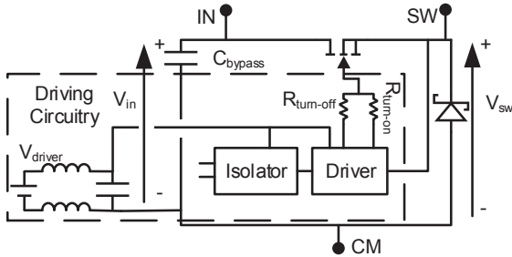
Fig. 2: Schematic of the Buck Cell
