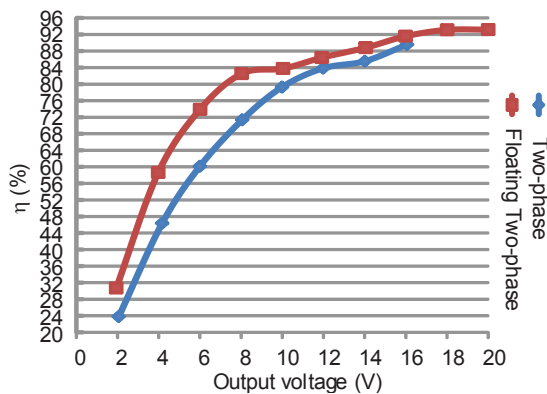
Fig. 22: Efficiency of the converters against output voltage
