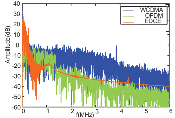
Fig. 25: Power spectral density of the envelopes used
