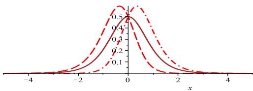
Fig. 3: Energy density of the solutions (h^{(+)}(x), A^{(-)}(x)) (dashed line) and (h^{(-)}(x), A^{(+)}(x)) (dashed-dotted line), and module of electric-charge density for both solutions (solid line).
