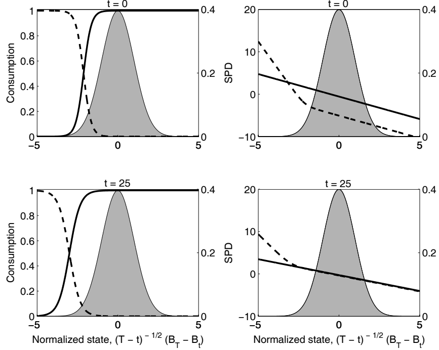
Figure 4: The terminal consumption of the rational and irrational traders as a fraction of the total consumption and the state price density (SPD) in different terminal states of the economy at different times. The model parameters are set to be \mu = 0.05 , \sigma = 0.15 , \eta = -4 , \gamma = 1 and T = 50 . The horizontal axis in all panels is the normalized state variable g_{t,T} \equiv (B_T - B_t)/\sqrt{T-t} , which has a standard normal distribution with zero mean and unit variance, which is shown by the shaded area (vertical axis on the right). In the two panels on the left, the terminal consumption for the rational trader (the solid line) and the irrational trader (the dotted line) are plotted against the normalized state variable at times t = 0, 25 , respectively, when B_t = 0 . In the two panels on the right, the dashed line plots the logarithm of the state price density at times t = 0, 25 , respectively, which is \ln \{[(1 + \xi_T)/D_T]/E_t [(1 + \xi_T)/D_T]\} . The solid line plots the logarithm of the state price density in the economy populated only by the rational traders, which is \ln \{D_T^{-1}/E_t [D_T^{-1}]\} .
