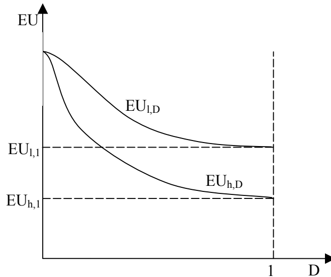
Figure 2: Expected utility as a function of deductible
