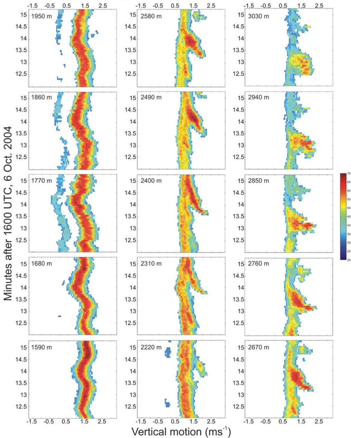
Figure 4: Doppler velocity power spectra at various heights over Barrow Alaska 6 October 2004. Each panel represents spectra at the stated height (indicated in the left upper corner) for the ~3 min period 1612 UTC to 1615 UTC. See text for discussion on the interpretation of the spectrographs.
