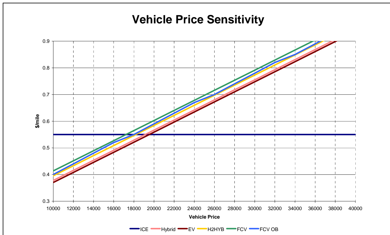
Figure 17. Vehicle Price Sensitivity
