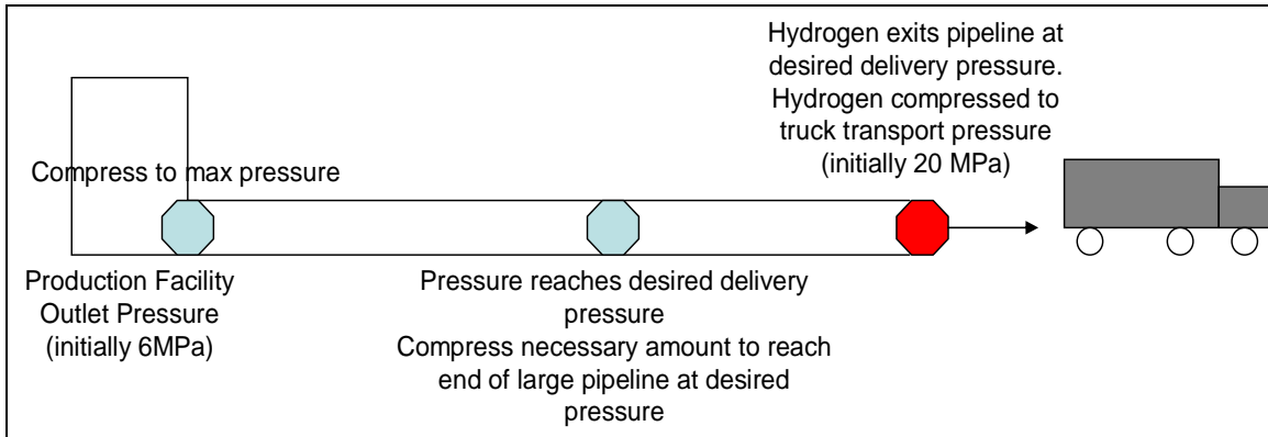
Figure 5. Large Pipelines and Local Truck Transport
