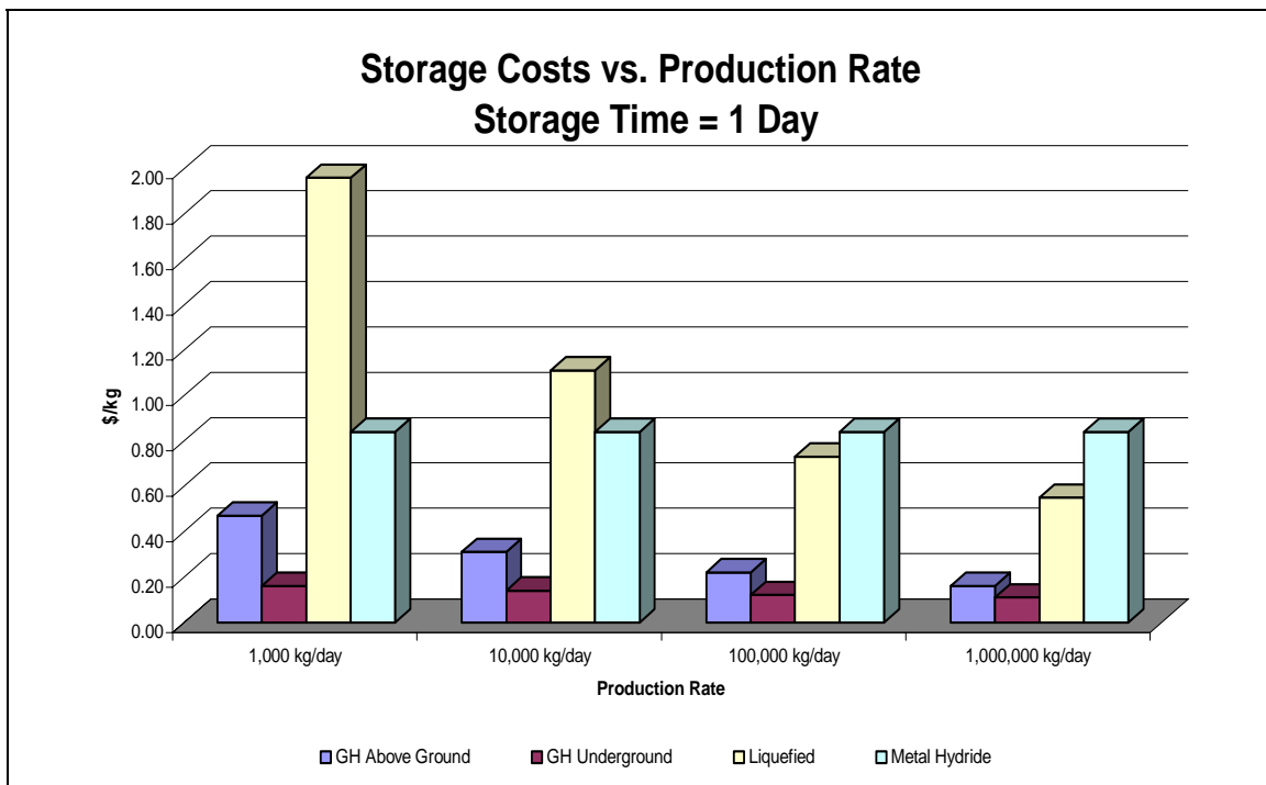
Figure 11. Storage Costs as a Function of Hydrogen Production Rate
