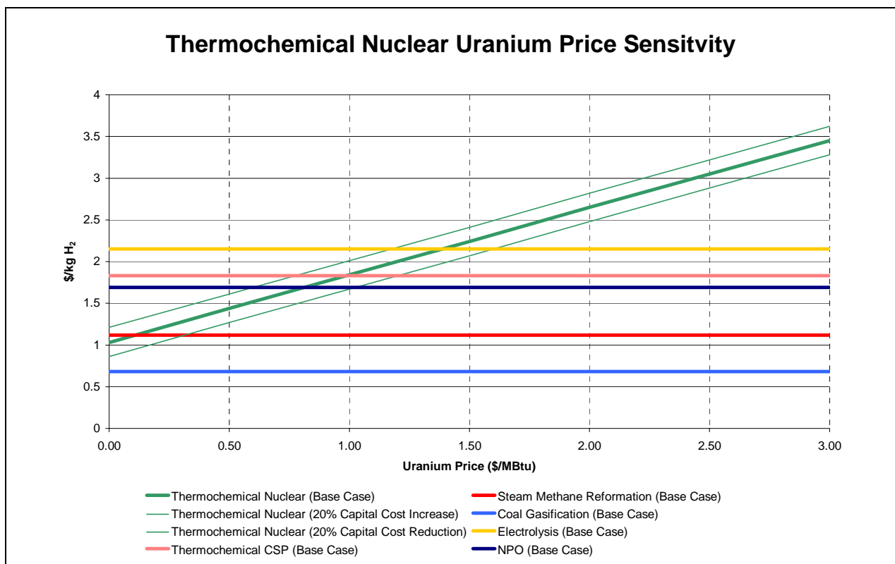
Figure 10. Thermochemical Nuclear Sensitivity to Uranium Prices
