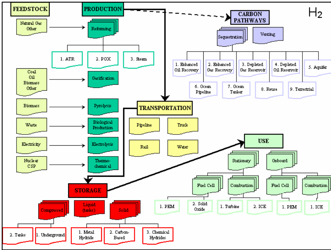
Figure 1. Hydrogen Pathways
