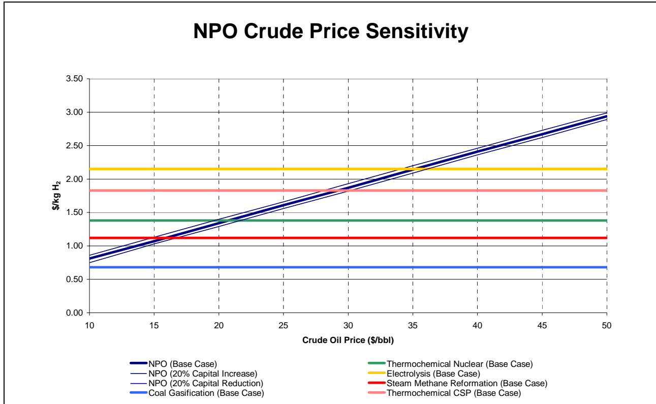
Figure 9. NPO Sensitivity to Crude Oil Prices
