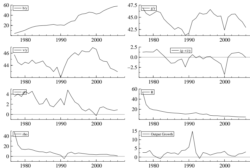
Figure 11: Germany data
