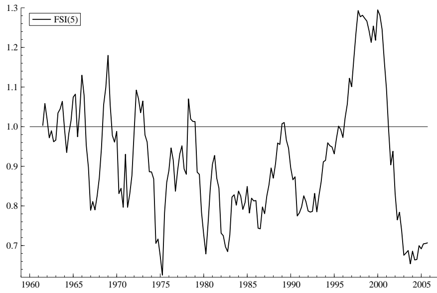
Figure 2.5: US FSI(5).
