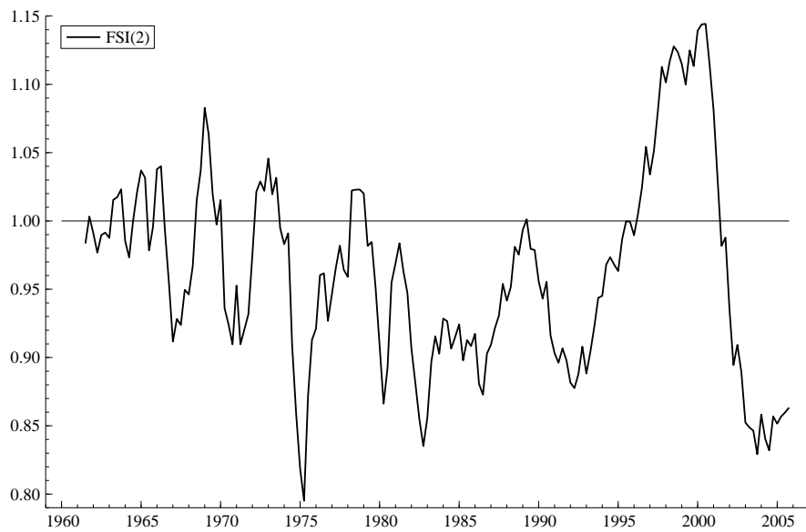
Figure 2.2: US FSI(2).
