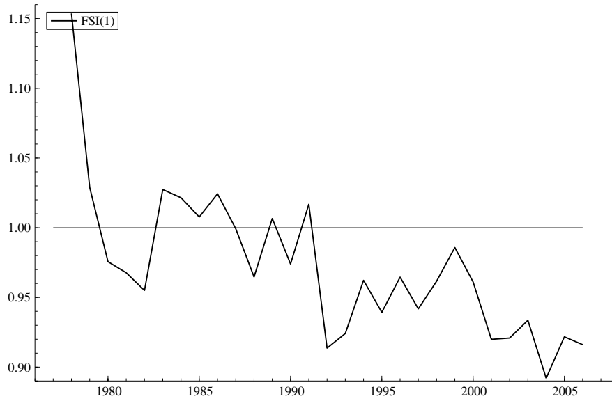
Figure 12: Germany FSI (1).
