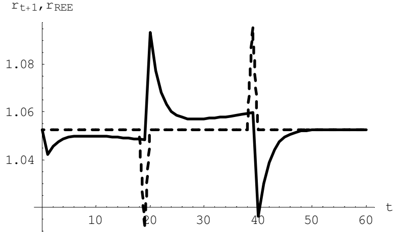
Figure 3: r_{t+1} under learning (solid line) and r_{REE} under rational expectations (dashed line), balanced-budget case with a temporary policy change.
