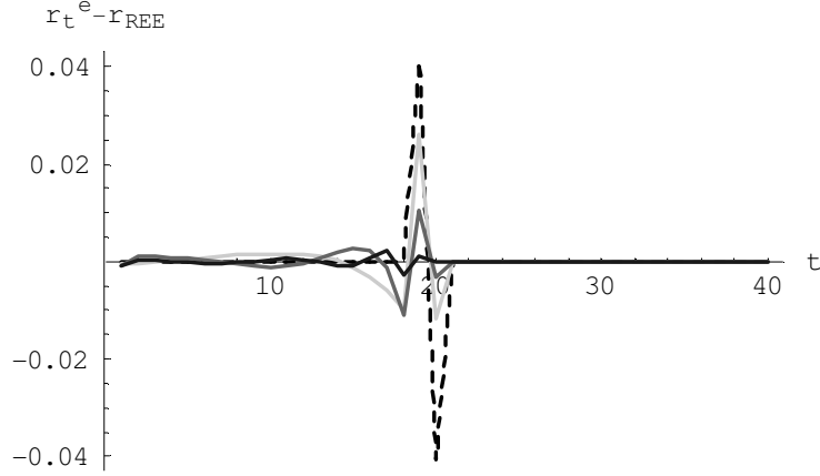
Figure 5: Difference between the RE values and the interest rate forecasts when the policy change is repeated. The differences are plotted for the second (dashed line), the 25th (solid light grey line), the 50th (solid medium grey line) and the 100th (solid black line) implementation. Note the convergence towards the RE values as the number of implementations increases.
