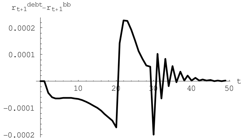
Figure 6: Difference between interest rates with debt financing and balanced budget, permanent policy change.
