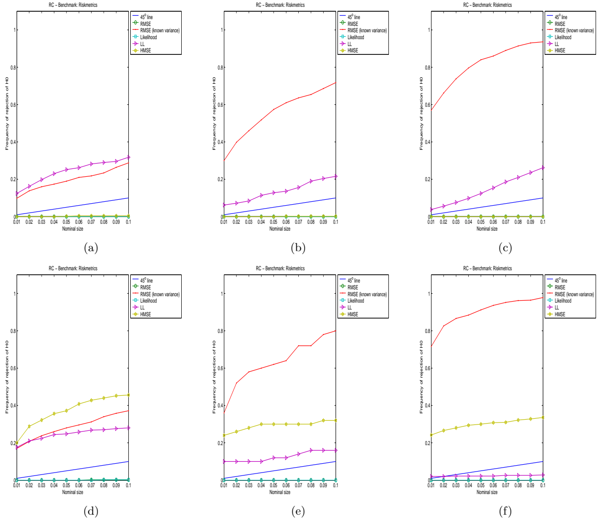
Figure 8: Frequencies of the cases where any of the concurrent models/methods are better than the benchmark for different significance levels of the Reality Check test when data are generated according Model 4. Panel (a) refers to 1000 observations. Panel (b) refers to 5000 observations. Panel (c) refers to 15000 observations. Panel (d) refers to 1000 observations with RM(0.85), MA(5), and MA(10) removed from the simulation. Panel (e) refers to 5000 observations with RM(0.85), MA(5), and MA(10) removed from the simulation. Panel (f) refers to 15000 observations with RM(0.85), MA(5), and MA(10) removed from the simulation.
