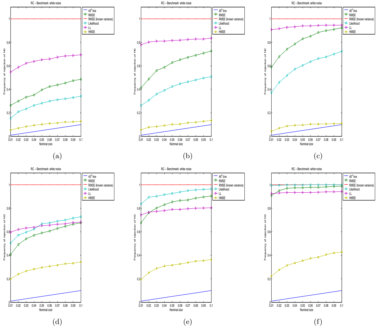
Figure 4: Frequencies of the cases where any of the concurrent models/methods are better than the benchmark for different significance levels of the Reality Check test when data are generated according Model 1. Panel (a) refers to 1000 observations. Panel (b) refers to 5000 observations. Panel (c) refers to 15000 observations. Panel (d) refers to 1000 observations with RM(0.85), MA(5), and MA(10) removed from the simulation. Panel (e) refers to 5000 observations with RM(0.85), MA(5), and MA(10) removed from the simulation. Panel (f) refers to 15000 observations with RM(0.85), MA(5), and MA(10) removed from the simulation.
