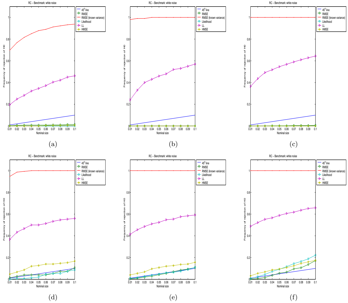
Figure 3: Frequencies of the cases where any of the concurrent models/methods are better than the benchmark for different significance levels of the Reality Check test when data are generated according Model 3. Panel (a) refers to 1000 observations. Panel (b) refers to 5000 observations. Panel (c) refers to 15000 observations. Panel (d) refers to 1000 observations with RM(0.85), MA(5), and MA(10) removed from the simulation. Panel (e) refers to 5000 observations with RM(0.85), MA(5), and MA(10) removed from the simulation. Panel (f) refers to 15000 observations with RM(0.85), MA(5), and MA(10) removed from the simulation.
