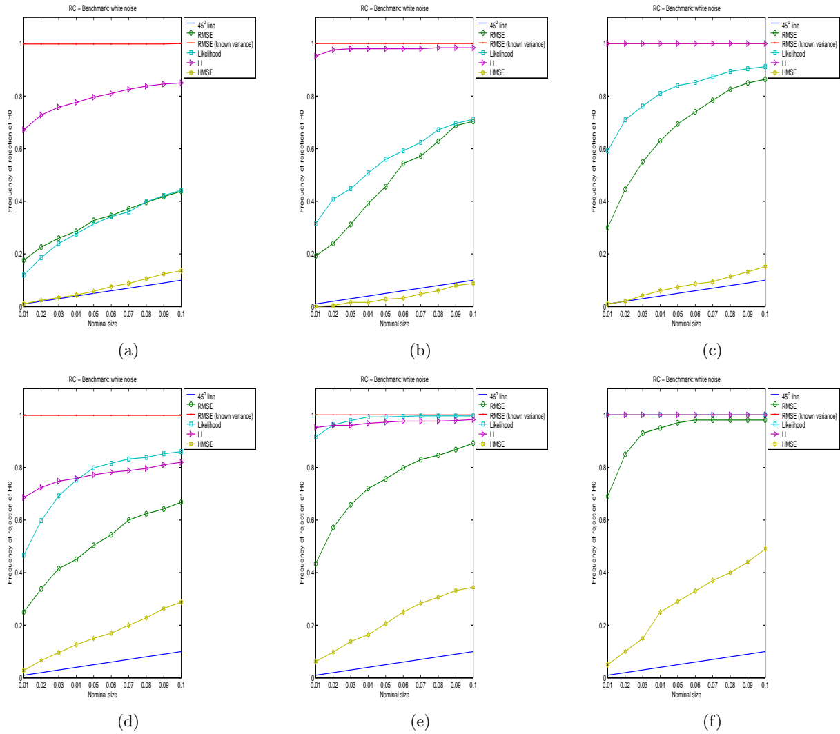
Figure 2: Frequencies of the cases where any of the concurrent models/methods are better than the benchmark for different significance levels of the Reality Check test when data are generated according Model 2. Panel (a) refers to 1000 observations. Panel (b) refers to 5000 observations. Panel (c) refers to 15000 observations. Panel (d) refers to 1000 observations with RM(0.85), MA(5), and MA(10) removed from the simulation. Panel (e) refers to 5000 observations with RM(0.85), MA(5), and MA(10) removed from the simulation. Panel (f) refers to 15000 observations with RM(0.85), MA(5), and MA(10) removed from the simulation.
