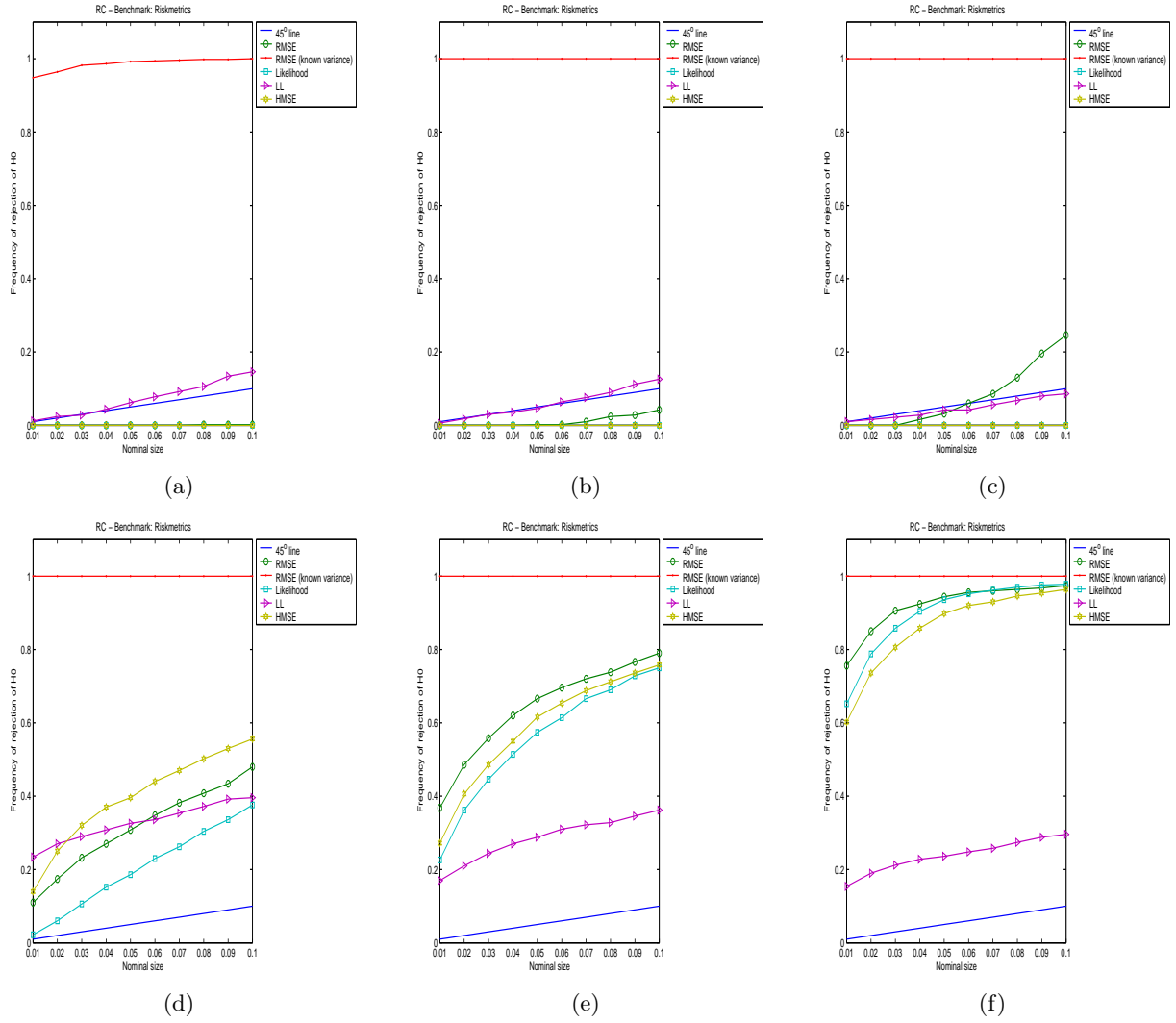
Figure 5: Frequencies of the cases where any of the concurrent models/methods are better than the benchmark for different significance levels of the Reality Check test when data are generated according Model 1. Panel (a) refers to 1000 observations. Panel (b) refers to 5000 observations. Panel (c) refers to 15000 observations. Panel (d) refers to 1000 observations with RM(0.85), MA(5), and MA(10) removed from the simulation. Panel (e) refers to 5000 observations with RM(0.85), MA(5), and MA(10) removed from the simulation. Panel (f) refers to 15000 observations with RM(0.85), MA(5), and MA(10) removed from the simulation.
