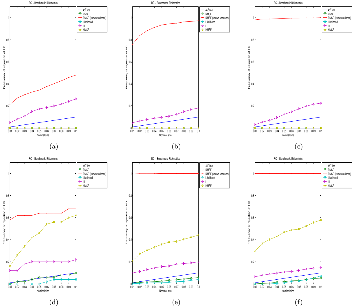
Figure 7: Frequencies of the cases where any of the concurrent models/methods are better than the benchmark for different significance levels of the Reality Check test when data are generated according Model 3. Panel (a) refers to 1000 observations. Panel (b) refers to 5000 observations. Panel (c) refers to 15000 observations. Panel (d) refers to 1000 observations with RM(0.85), MA(5), and MA(10) removed from the simulation. Panel (e) refers to 5000 observations with RM(0.85), MA(5), and MA(10) removed from the simulation. Panel (f) refers to 15000 observations with RM(0.85), MA(5), and MA(10) removed from the simulation.
