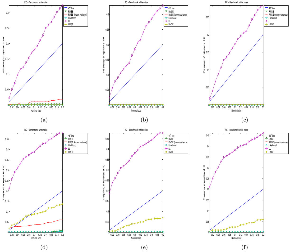
Figure 1: Frequencies of the cases where any of the concurrent models/methods are better than the benchmark for different significance levels of the Reality Check test when data are generated according Model 1. Panel (a) refers to 1000 observations. Panel (b) refers to 5000 observations. Panel (c) refers to 15000 observations. Panel (d) refers to 1000 observations with RM(0.85), MA(5), and MA(10) removed from the simulation. Panel (e) refers to 5000 observations with RM(0.85), MA(5), and MA(10) removed from the simulation. Panel (f) refers to 15000 observations with RM(0.85), MA(5), and MA(10) removed from the simulation.
