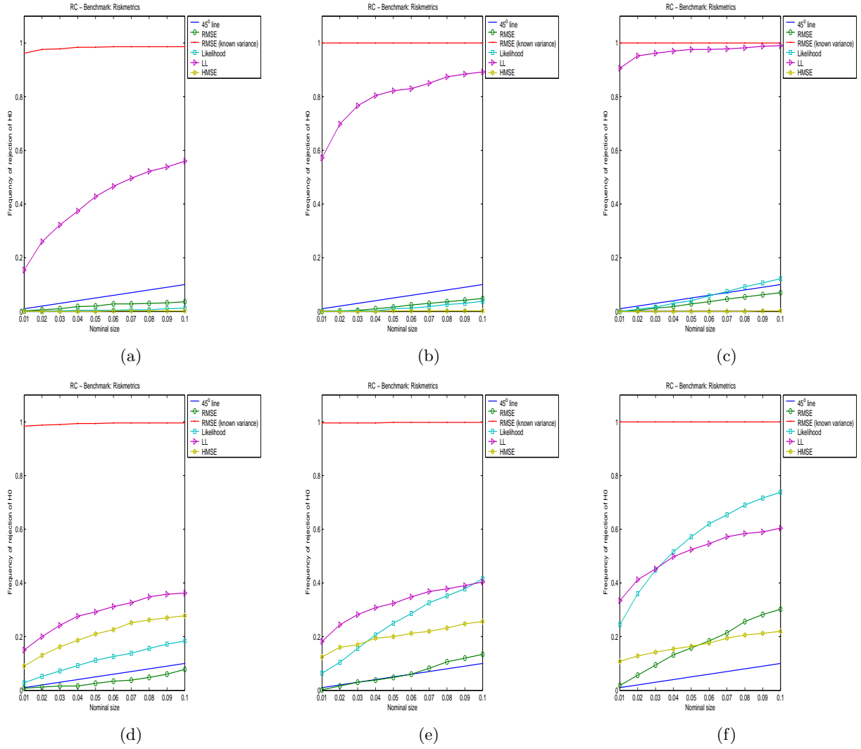
Figure 6: Frequencies of the cases where any of the concurrent models/methods are better than the benchmark for different significance levels of the Reality Check test when data are generated according Model 2. Panel (a) refers to 1000 observations. Panel (b) refers to 5000 observations. Panel (c) refers to 15000 observations. Panel (d) refers to 1000 observations with RM(0.85), MA(5), and MA(10) removed from the simulation. Panel (e) refers to 5000 observations with RM(0.85), MA(5), and MA(10) removed from the simulation. Panel (f) refers to 15000 observations with RM(0.85), MA(5), and MA(10) removed from the simulation.
