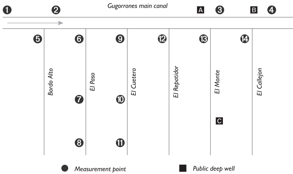
FIGURE 2B. Schematic representation of measurement points in the Gugorrones main canal, in the Salvatierra module.
