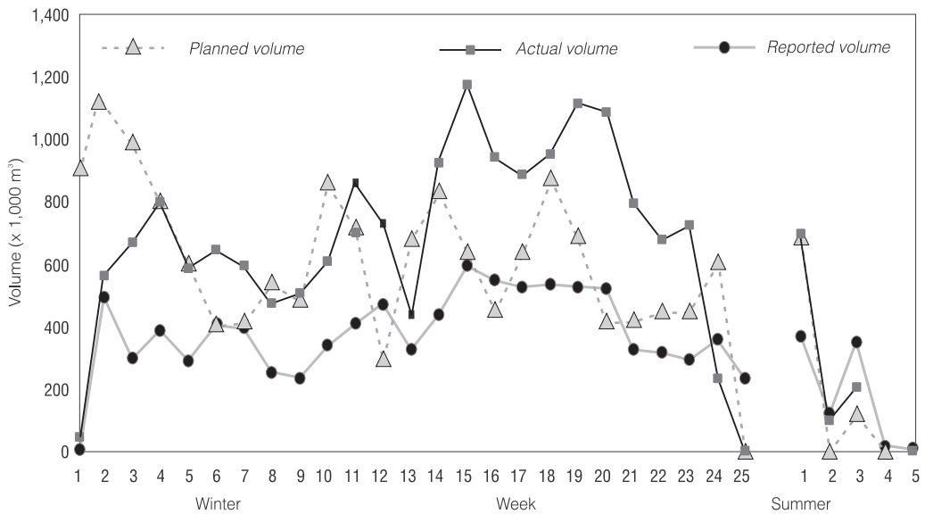
FIGURE 3C. Planned, actual, and reported volumes of the Gugorrones main canal, in the Salvatierra module, in winter and summer seasons, 1995–96.
