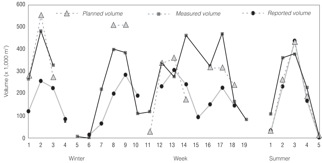
FIGURE 3B. Planned, actual, and reported volumes of lateral B of the Cortazar module, in winter and summer seasons, 1995–96.
