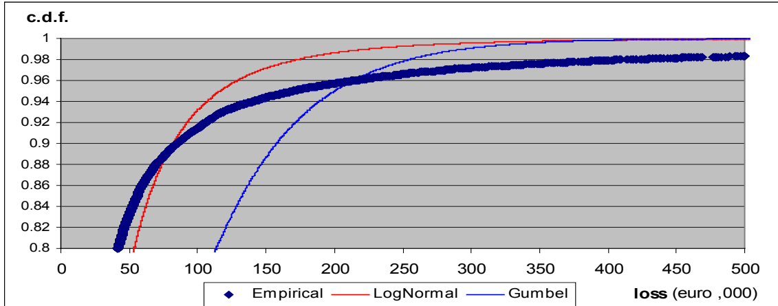
Figure 4: BL 3 (Retail Banking). LogNormal and Gumbel fit (focus on the tail)
