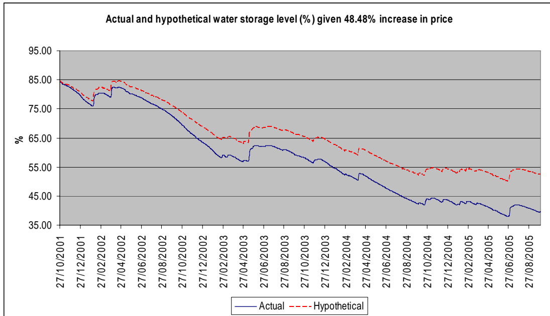
Figure 2: Actual and Hypothetical Water Storage over 2001-2005 Period.
