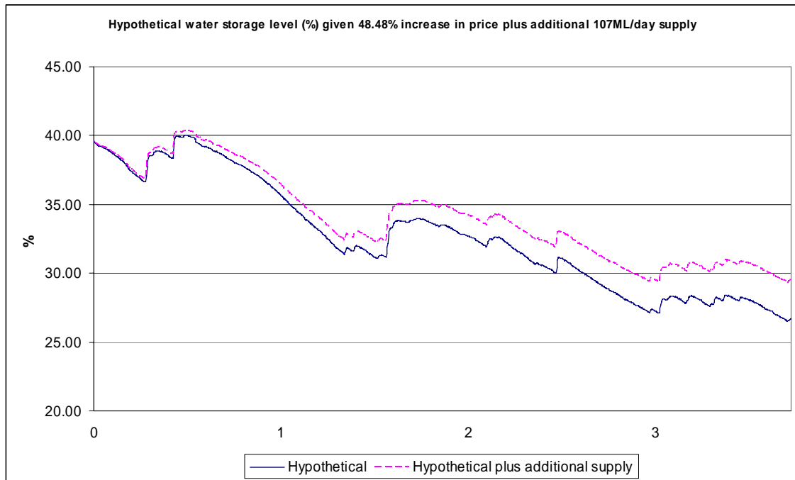
Figure 4: Hypothetical Water Storage Levels with 48.48% Increase Above IPART Scheduled Prices Plus Additional Water Supplies of 107 Mega Litres/day or approx. 39 GL/year — Four Year projection.
