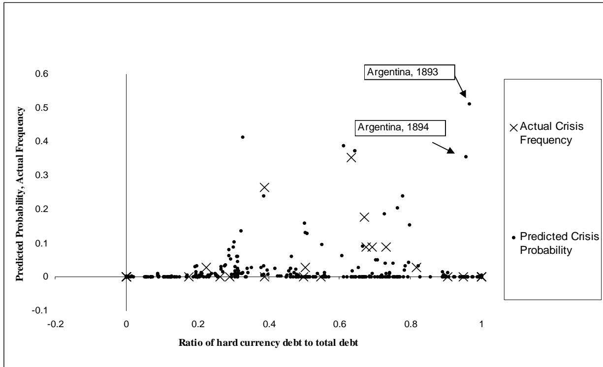
Figure 12 Actual and Predicted Debt Crisis Frequencies versus the Ratio of Hard Currency Public Debt to Total Public Debt, 1880-1913
