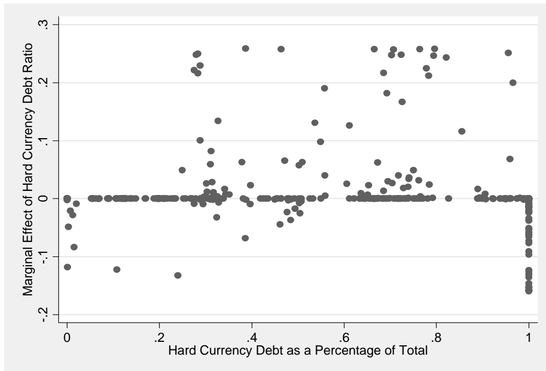
Figure 10 Marginal Effect of the Ratio of Hard Currency Debt to Total Debt
