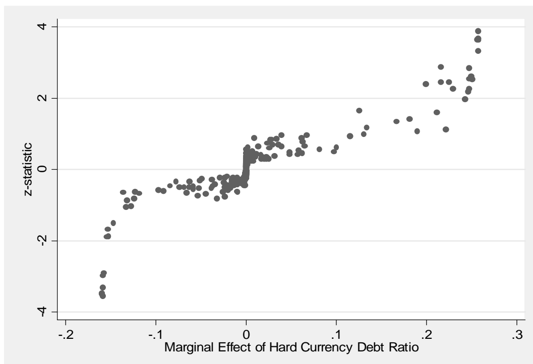
Figure 11 Z-Statistics by Observation from a Test of the Hypothesis that the Marginal Effect is Zero
