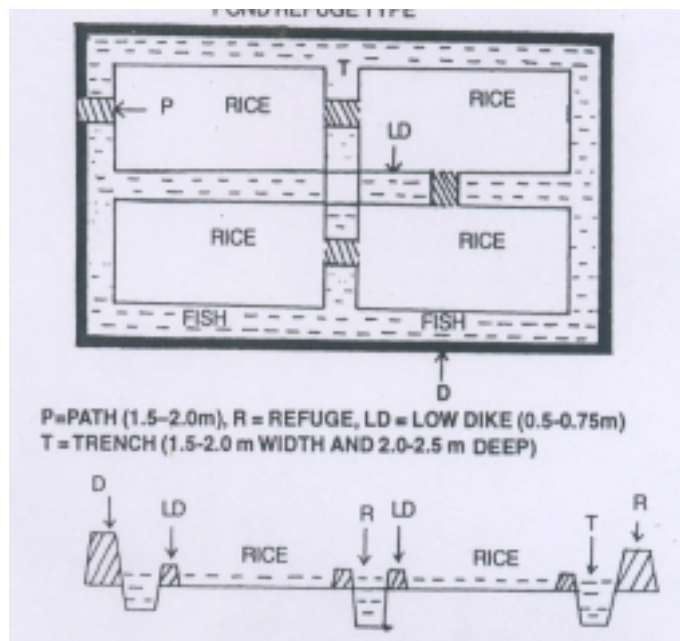
Fig.2 Field diagrams of combined fish-cum-rice/other crop culture
