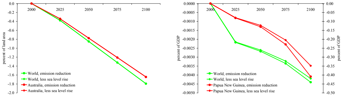
Figure 8. The effects of lower sea level rise alone and of emission reduction on wetland loss (left panel) and its costs (right panel) for the world (left axis) and for Australia (wetland area) and Papua New Guinea (wetland costs; right axis).
