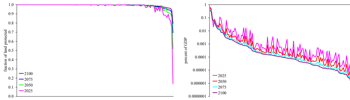
Figure 3. Protection level (fraction of coast protected; left panel) and the costs of protection (percent of GDP; right panel). Countries are ranked as to their protection level.
