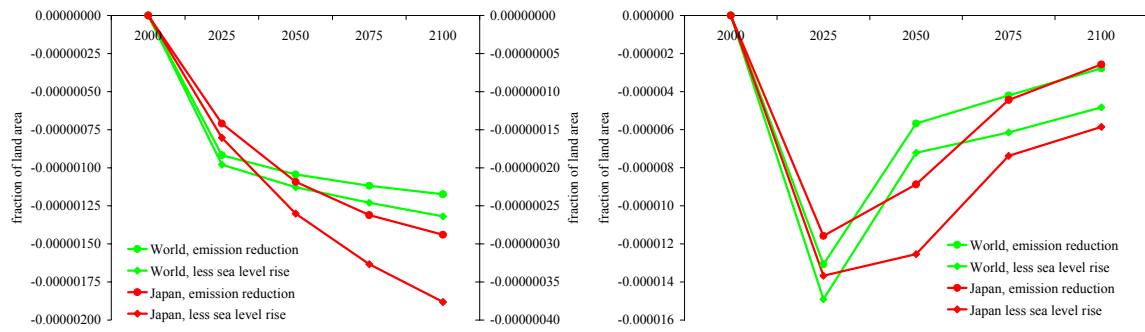
Figure 6. The effects of lower sea level rise alone and of emission reduction on dryland loss (left panel) and its costs (right panel) for the world (left axis) and for Japan (right axis).
