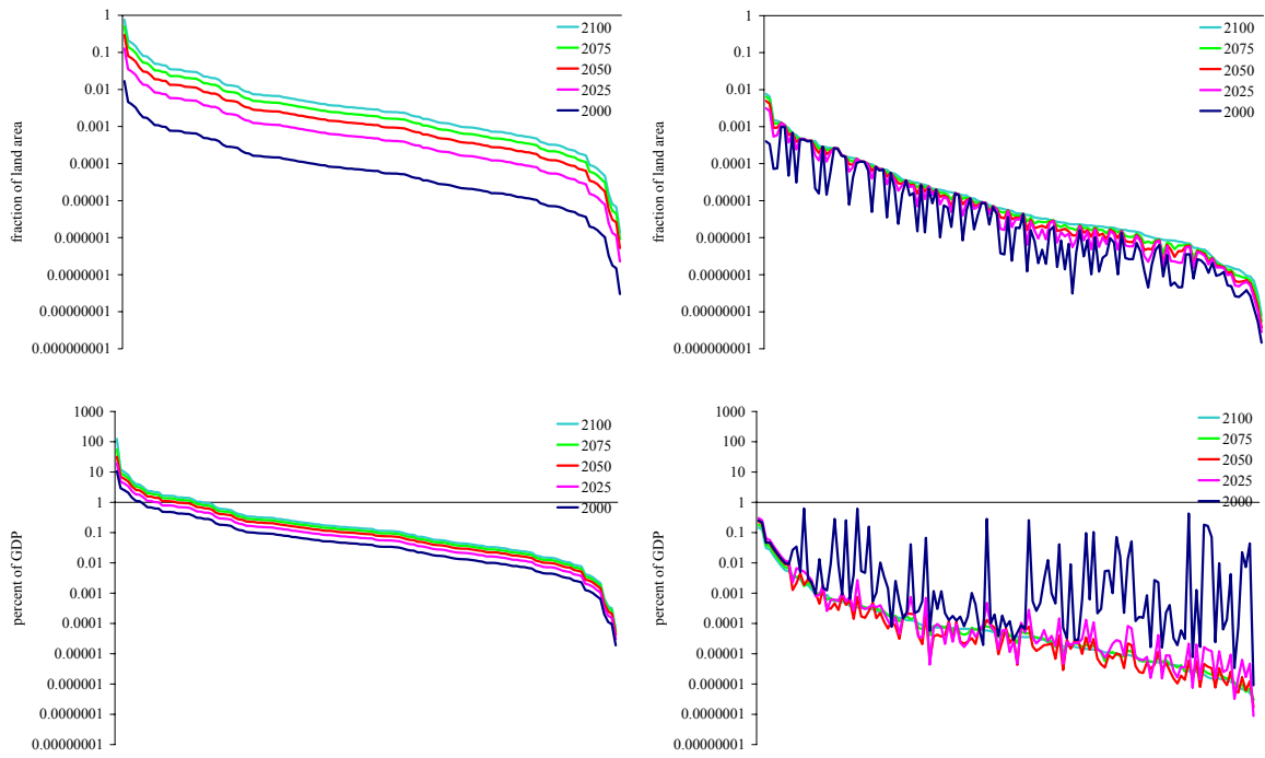
Figure 1. Loss of dryland (fraction of total area in 2000; top panels) and its value (percent of GDP; bottom panels) without protection (left panels) and with (right panels). Countries are ranked as to their values in 2100.
