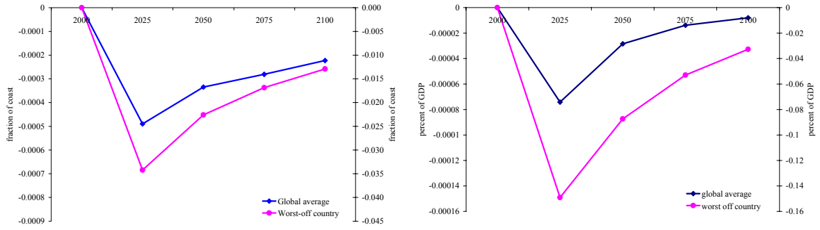
Figure 4. The effects of lower sea level rise and emission reduction costs on coastal protection for the world and for Kiribati (left panel) and on the costs of coastal protection for the world and for Micronesia (right panel).
