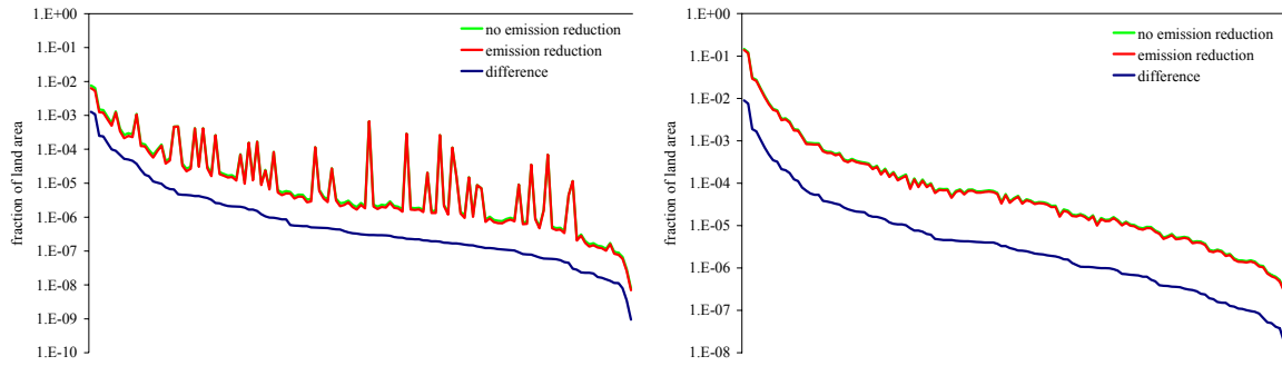
Figure 5. The dryland loss (fraction of 2000 land area; left panel) and its costs (percent GDP; right panel) in 2100 according to the business as usual scenario and the emission reduction scenario. The difference is also shown. Countries are ranked according to the difference.
