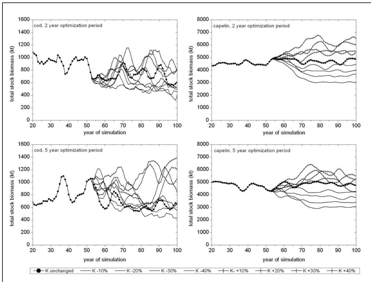
Figure 2. Development of the stock sizes with altered carrying capacities.
