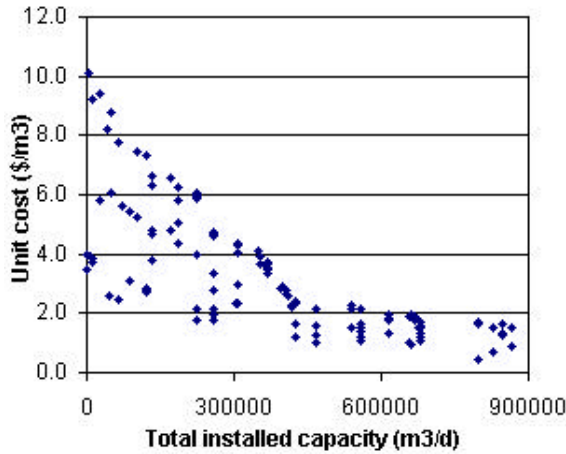
Fig. 6. Unit costs by the ME process.
