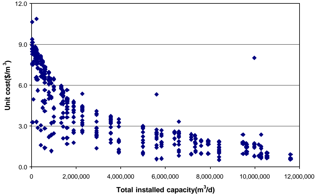
Fig. 3. Unit costs vs. total installed capacity by the MSF process.
