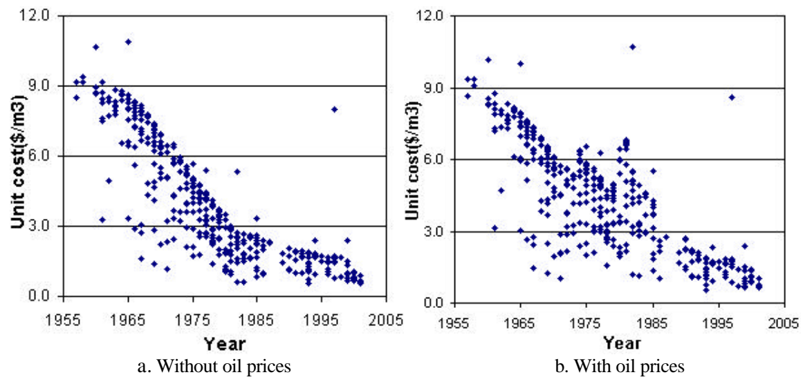
Fig. 4. Sensitivity analysis of unit costs regarding energy costs.
