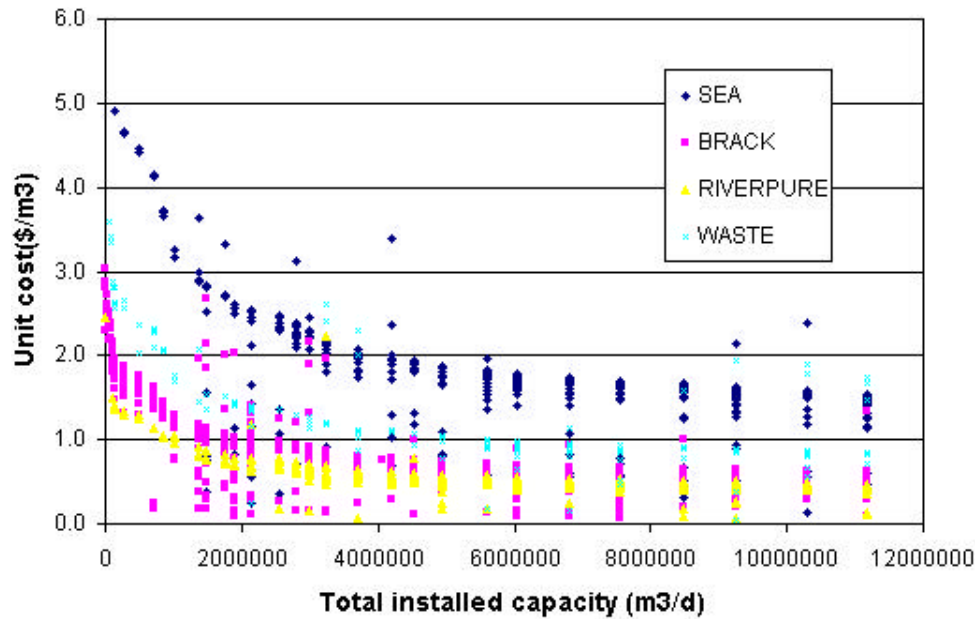
Fig. 5. Unit costs vs. total installed capacity by the RO process.
