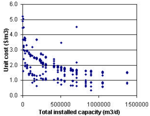
Fig. 7. Unit costs by the VC process.
