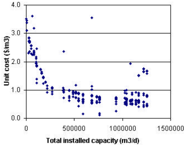
Fig. 8. Unit costs by the ED process.
