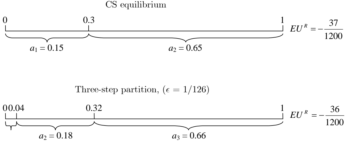
Figure 2: Equilibria with b = \frac{1}{10}
