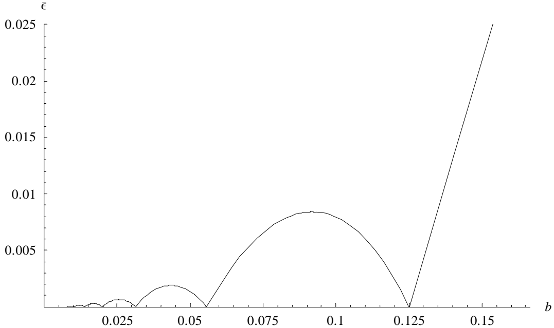
Figure 4: \epsilon^* as a function of b
