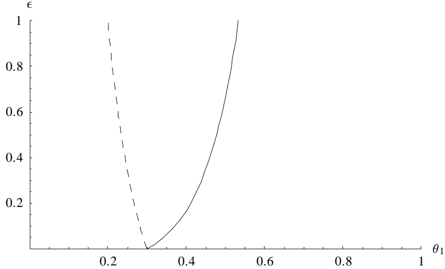
Figure 1: Two-step equilibrium partitions, b = \frac{1}{10} .
