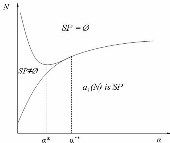
Figure 4: The set of Secession-proof fees
