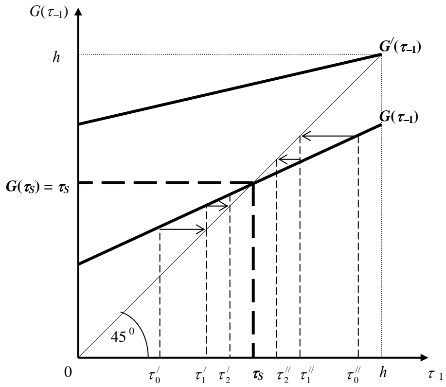
Figure 2. The Existence of a Stationary Protection Sequence at \tau_S
