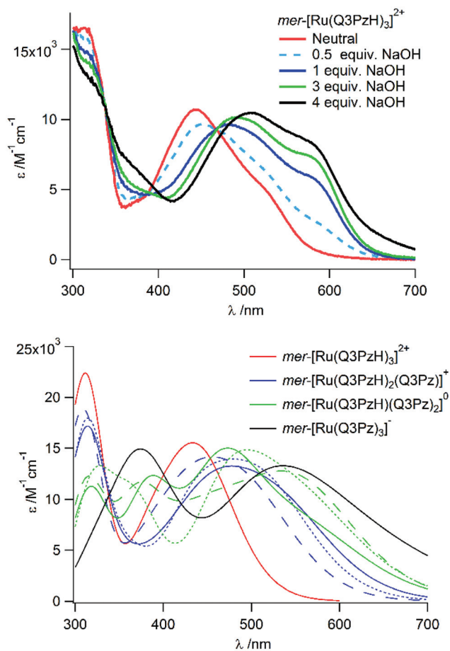
Fig. 4 (Top panel) Titration of NaOH to mer-[Ru(Q3PzH)_3]^{2+} in MeCN and (bottom panel) calculated absorption spectra with 0.25 eV broadening of all of the possible protonation states of mer-[Ru(Q3PzH)_{3-x}(Q3Pz^-)_x]^{(2-x)+} in acetonitrile ( x = 0-3 ), where the lowest energy spectra of each protonation state is shown as a solid line.
