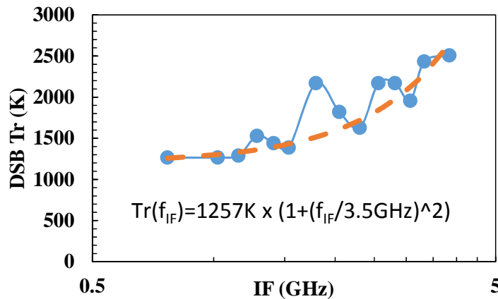
Figure 5. The measured DSB receiver noise temperature for the Herschel FM03 NbN HEB mixer at 1.63THz LO. No corrections for the optical loss were applied. Bias: 1mV, 47μA. The noise temperature is very similar to the one measured with the same sample prior to the delivery in 2005. A different IF LNA was used this time (0.1-5GHz) which allows for measurements from lower IFs. The mixer unit itself has a lower cut-off frequency at 500GHz (the built-in bias-T).
