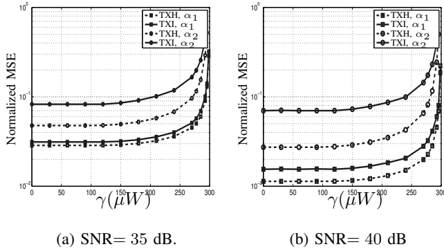
Fig. 1: Error versus energy harvesting requirements
