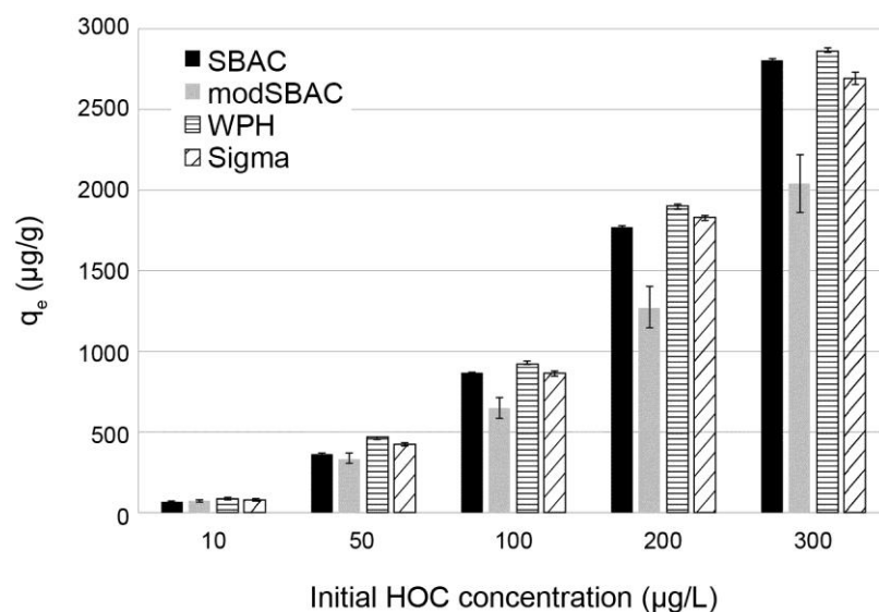
Figure 2. Adsorption capacity ( q_e ) of HOCs on sewage-based activated carbon (SBAC) and surface-modified SBAC (modSBAC), as well as commercial activated carbons WPH and Sigma. Plotted q_e :s are mean of duplicate samples and error bars indicate standard error of q_e at each spike level.
