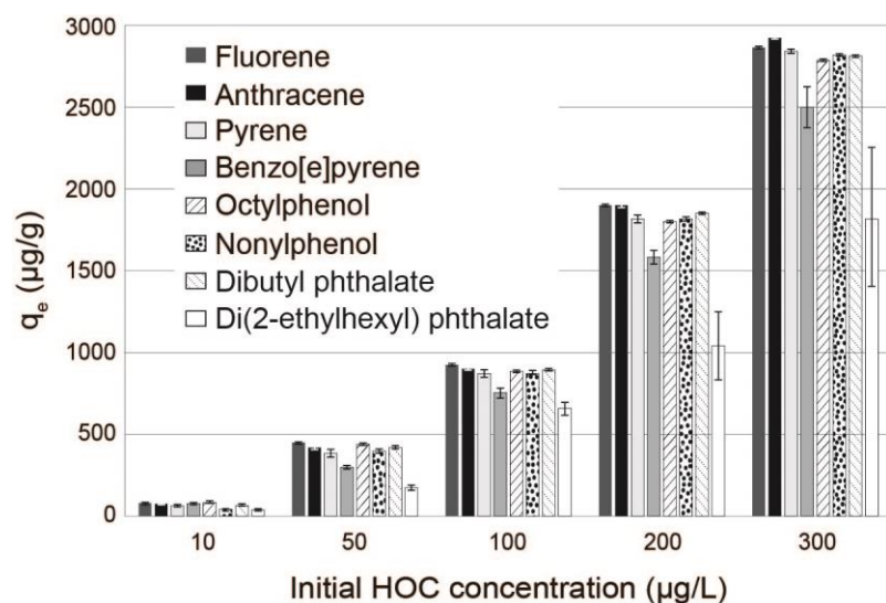
Figure 3. Adsorption capacity ( q_e ) of HOCs using SBAC at C_{initial}=10-300 \mu\text{g/L} . Plotted q_e 's are mean of duplicate samples and error bars indicate standard error of q_e .
