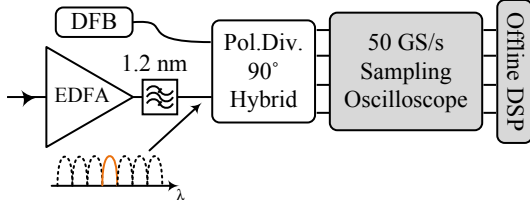
Fig. 4: Schematics of the coherent receiver.
