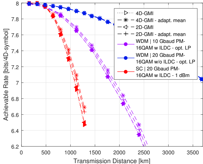
Fig. 14: Achievable rates for 4D and 2D GMI, with and without adaptive mean values of the received constellation.
