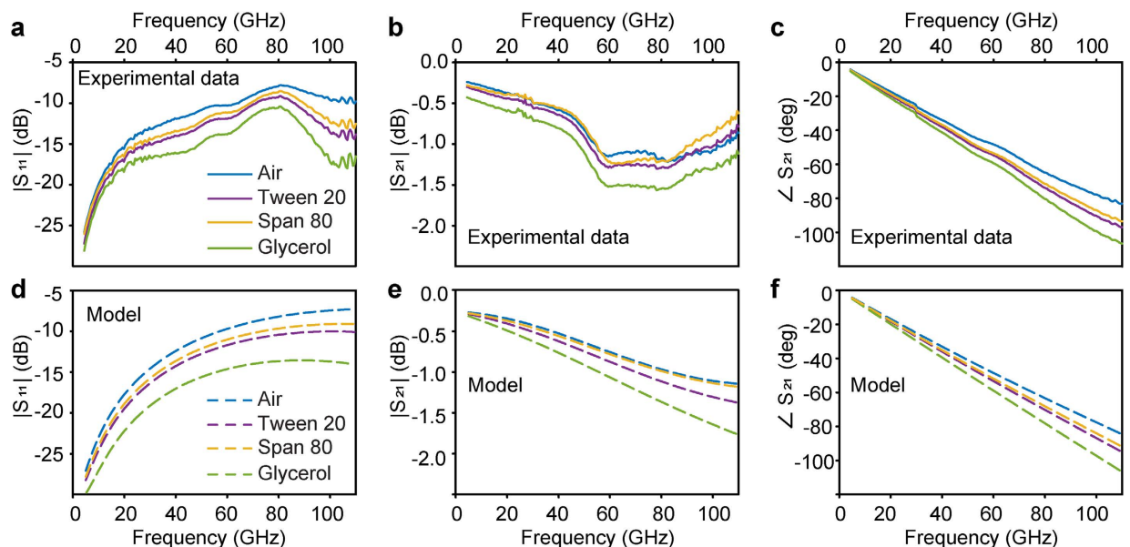
Figure 5. Comparison of the experimental data after the de-embedding process (a–c, continuous lines) and the circuit model with adjusted values of the permittivity (d–f, dashed lines). The magnitude of S_{11} (a,d), S_{21} (b,e) and the phase of S_{21} (c,f). Air (blue), Tween 20 (purple), Span 80 (yellow) and glycerol (green).
